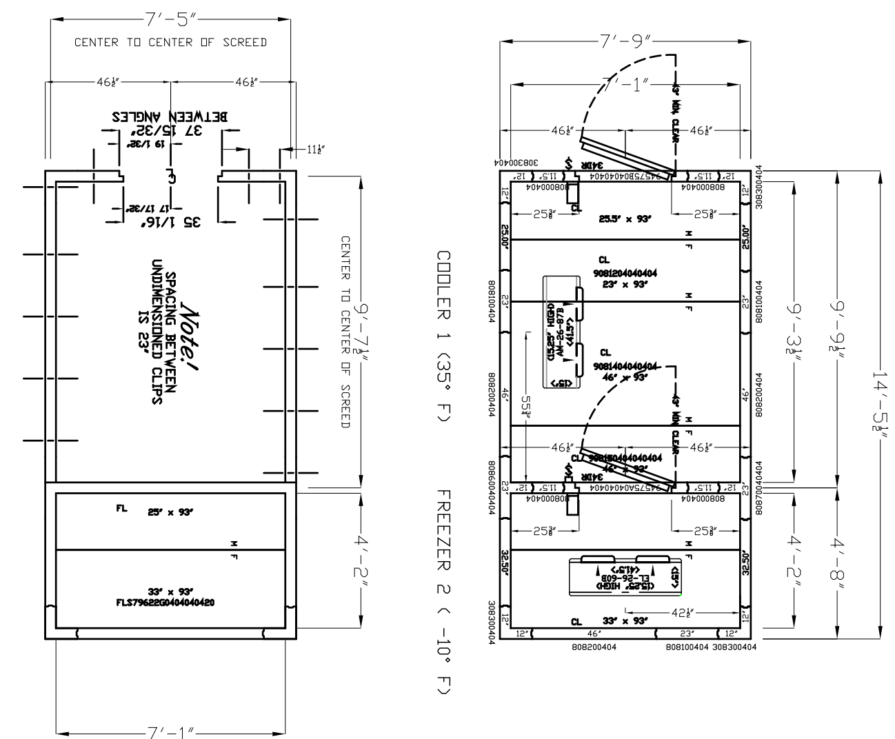
4" X 4" (HIGH) VINYL FOAM SCREED AND FLOOR PANEL LAYOUT
