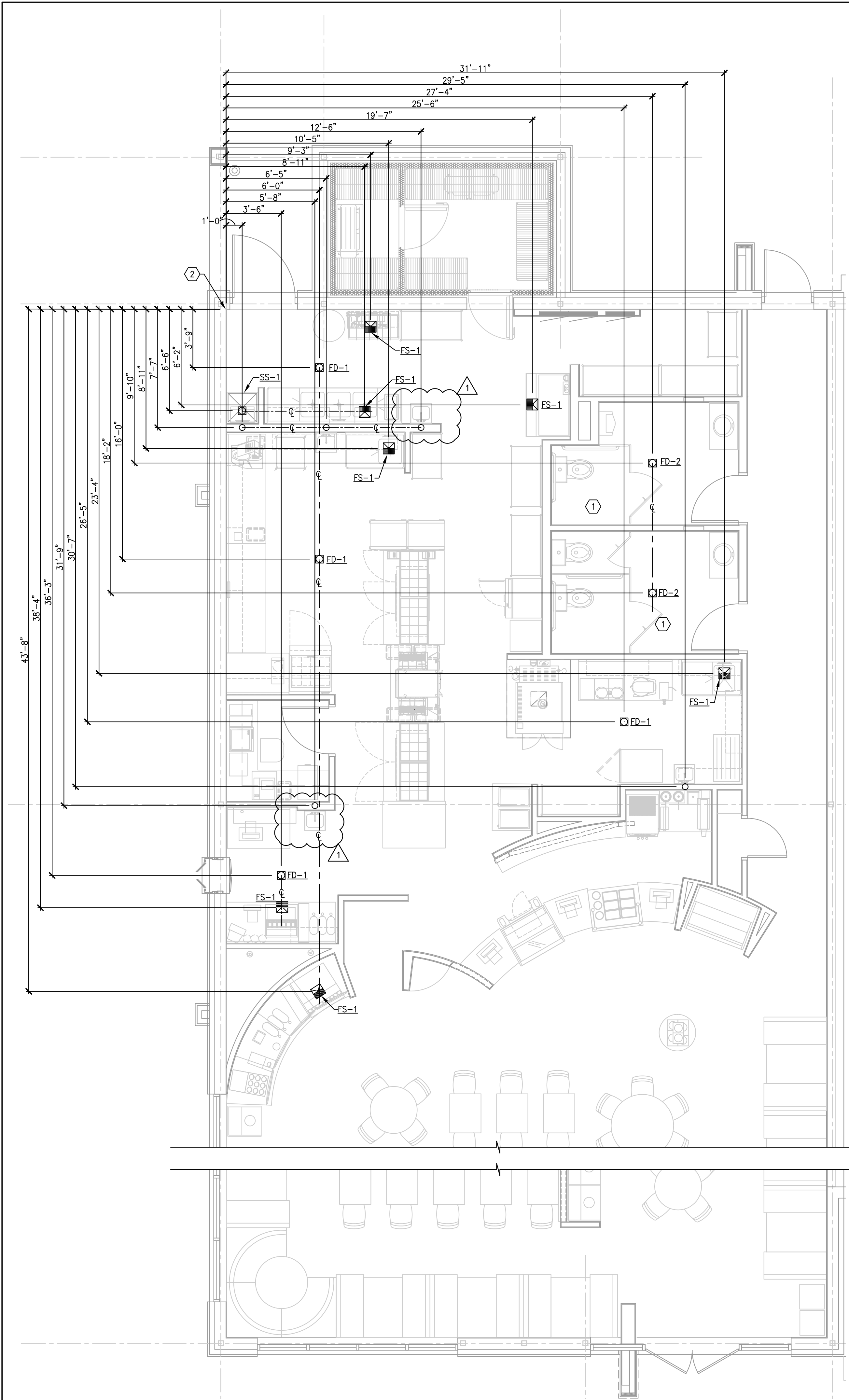
UNDERSLAB ROUGH-IN PLAN SCALE: 1/4"=1'-0"
