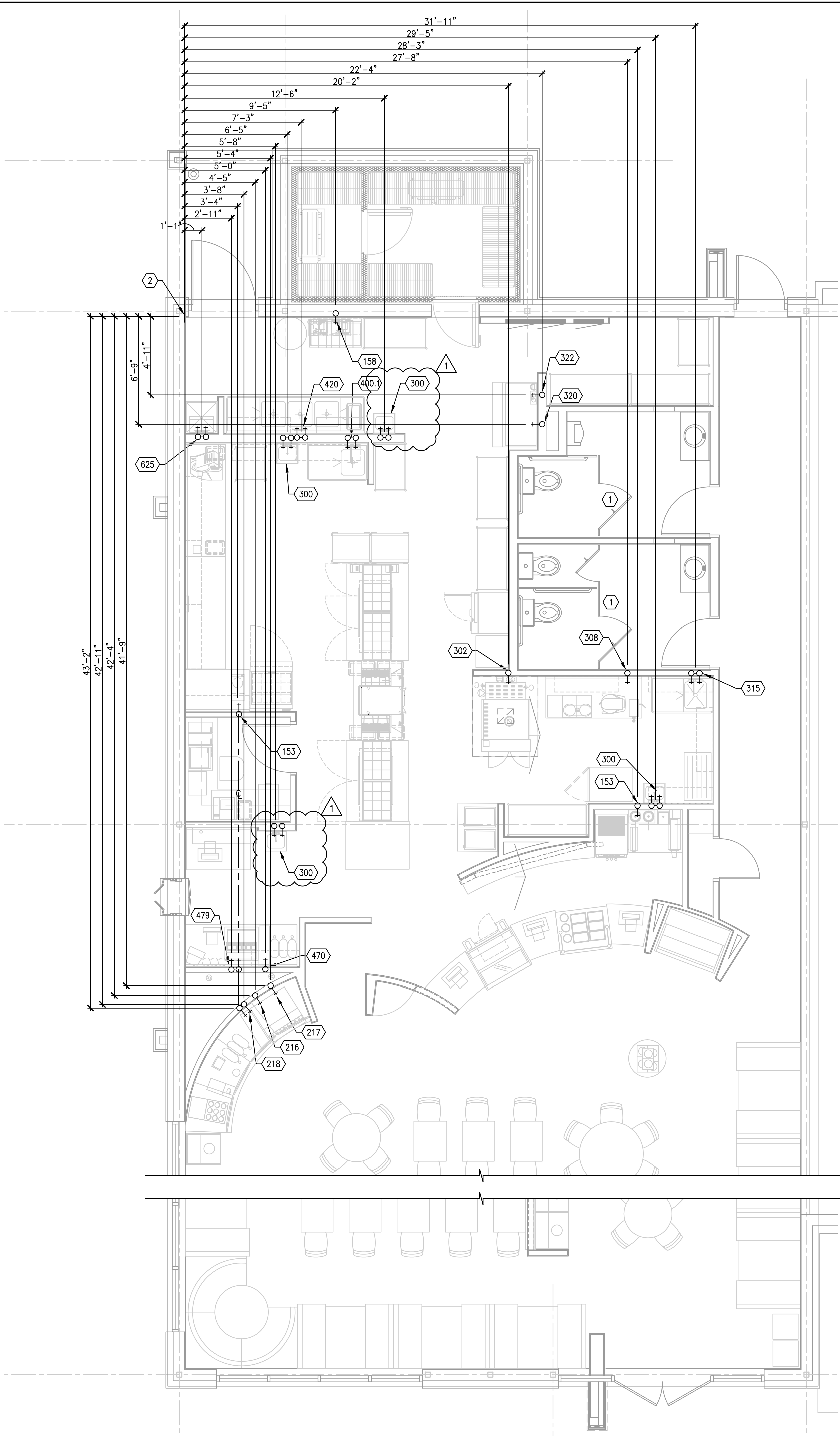
WATER ROUGH-IN PLAN SCALE: 1/4"=1'-0"
