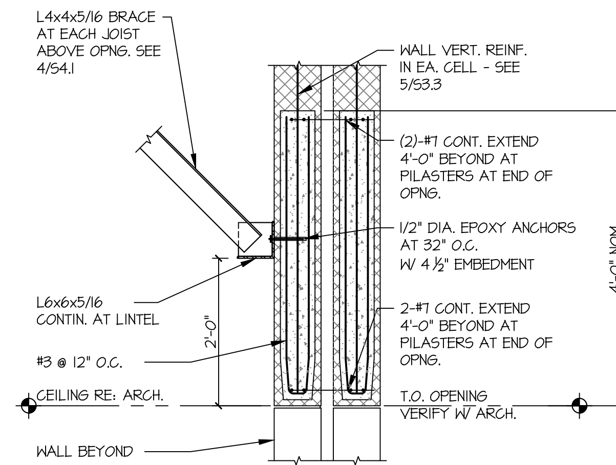
TYPICAL DETAIL @ CMU LINTEL AT OPENING
