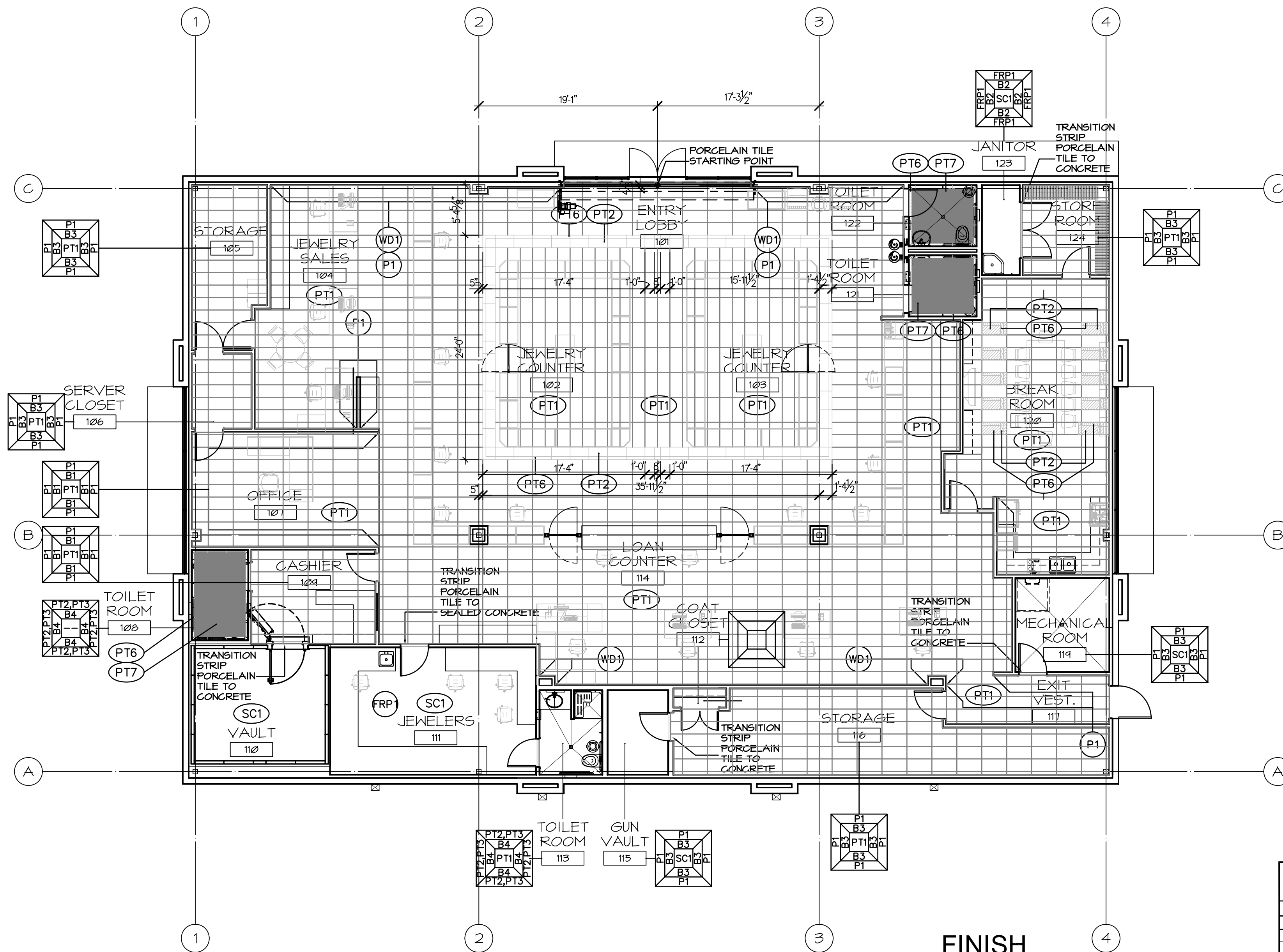
1 FINISH FLOOR PLAN A9.1 SCALE: 1/8" = 1'-0"
