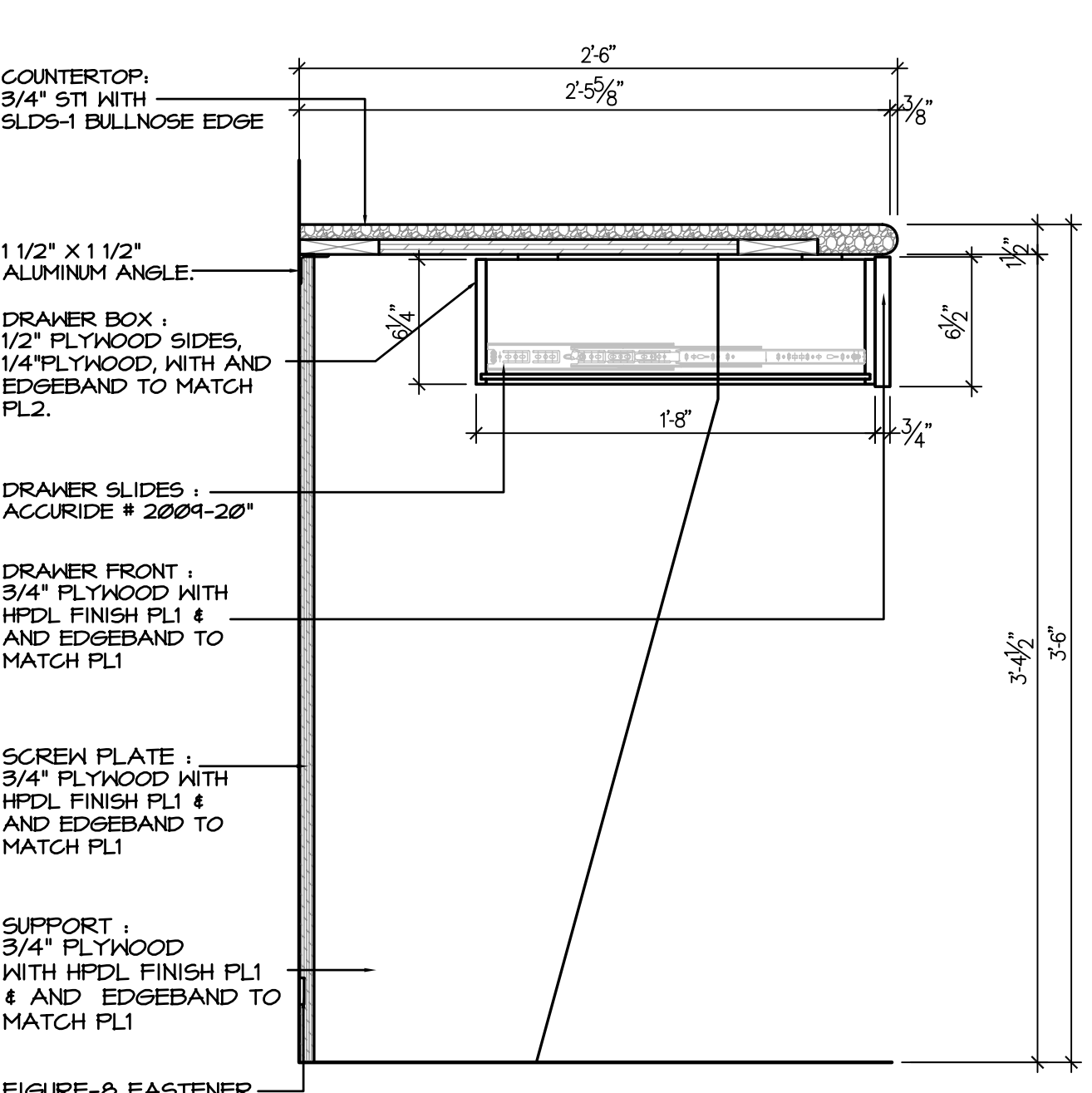
8 MILLWORK SECTION A7.4 SCALE: 1 1/2" = 1'-0"
