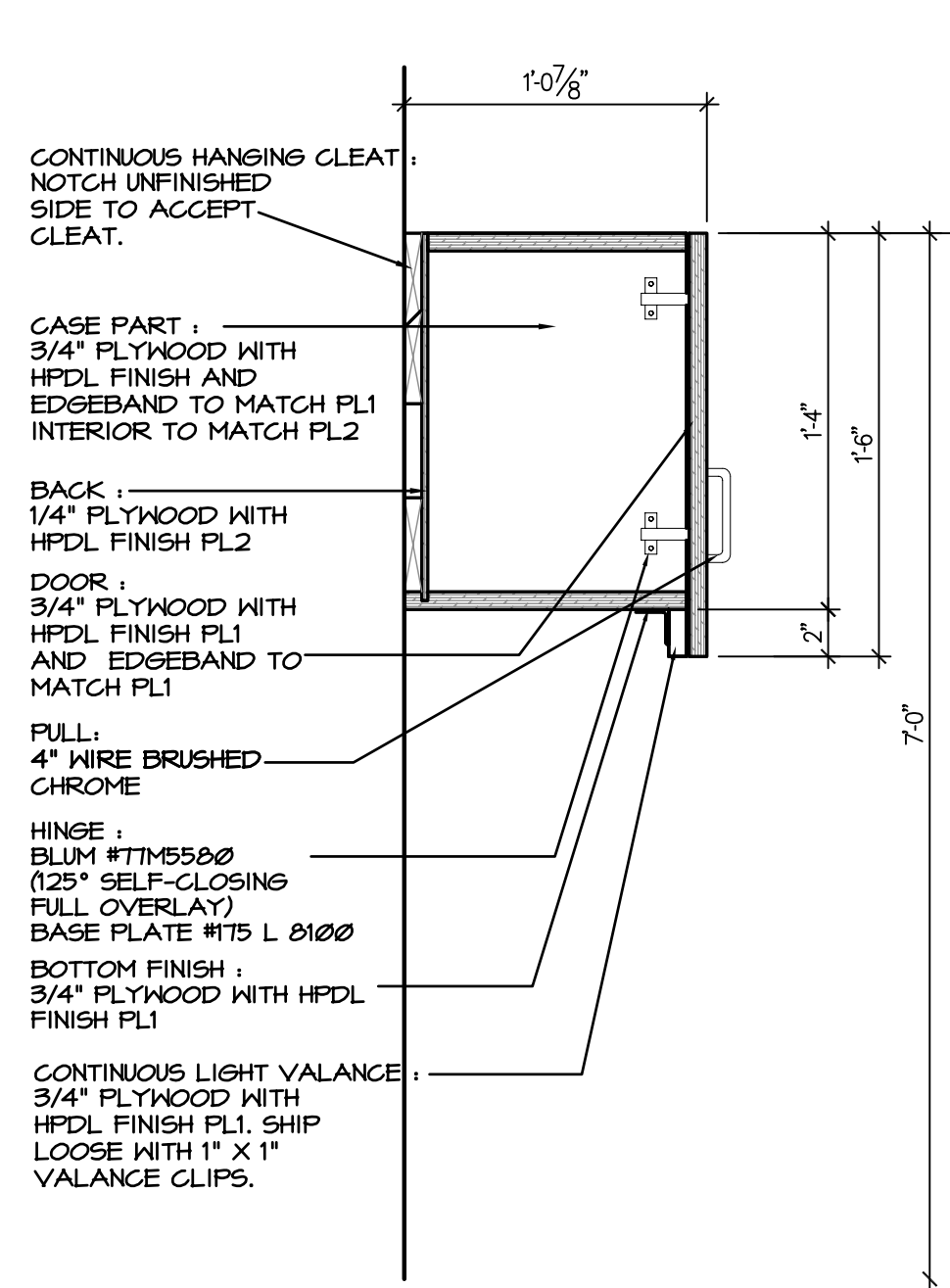
1 MILLWORK SECTION A7.4 SCALE: 1 1/2" = 1'-0"
