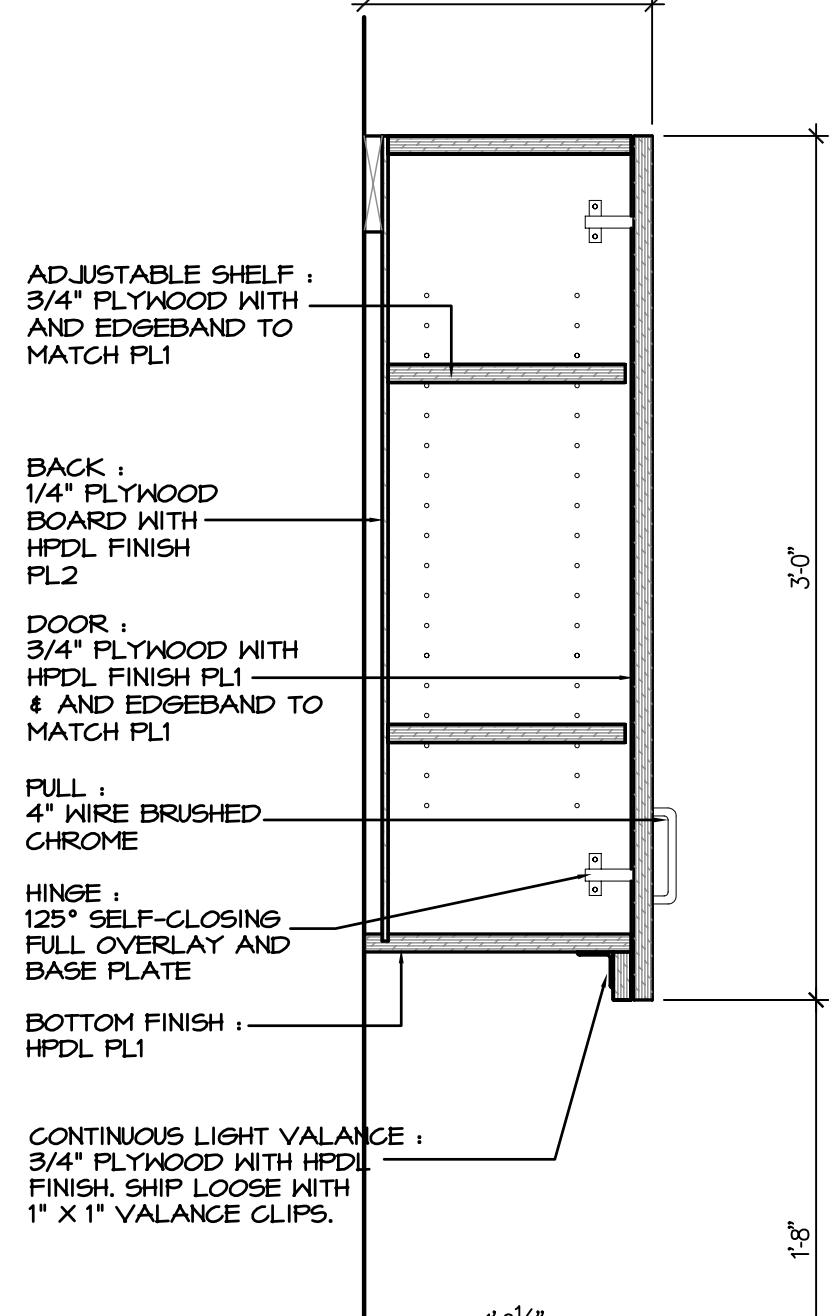
8 MILLWORK SECTION A7.4 SCALE: 1 1/2" = 1'-0"
