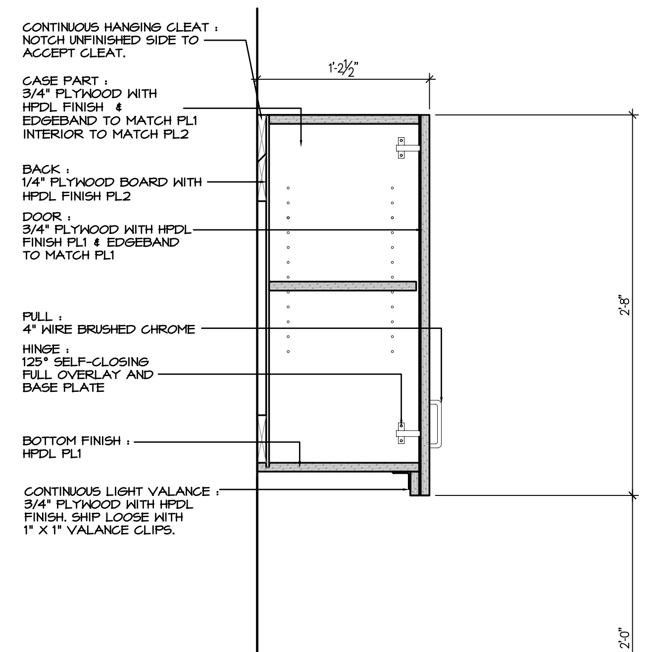
7 MILLWORK SECTION A7.4 SCALE: 1 1/2" = 1'-0"
