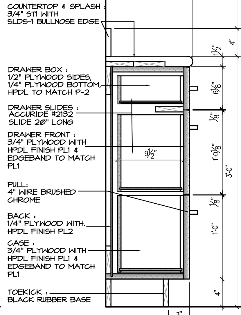
3 MILLWORK SECTION A7.4 SCALE: 1 1/2" = 1'-0"
