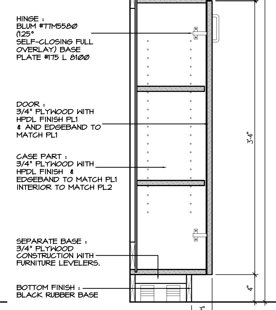
4 MILLWORK SECTION A7.4 SCALE: 1 1/2" = 1'-0"
