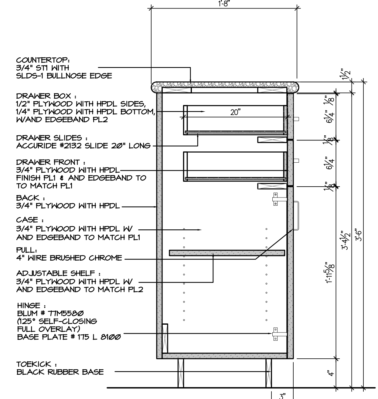
9 MILLWORK SECTION A7.4 SCALE: 1 1/2" = 1'-0"
