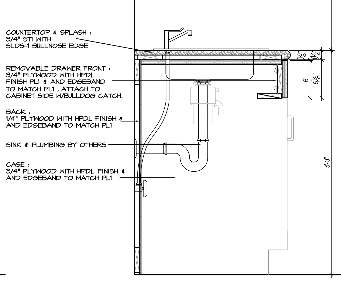
2 MILLWORK SECTION A7.4 SCALE: 1 1/2" = 1'-0"
