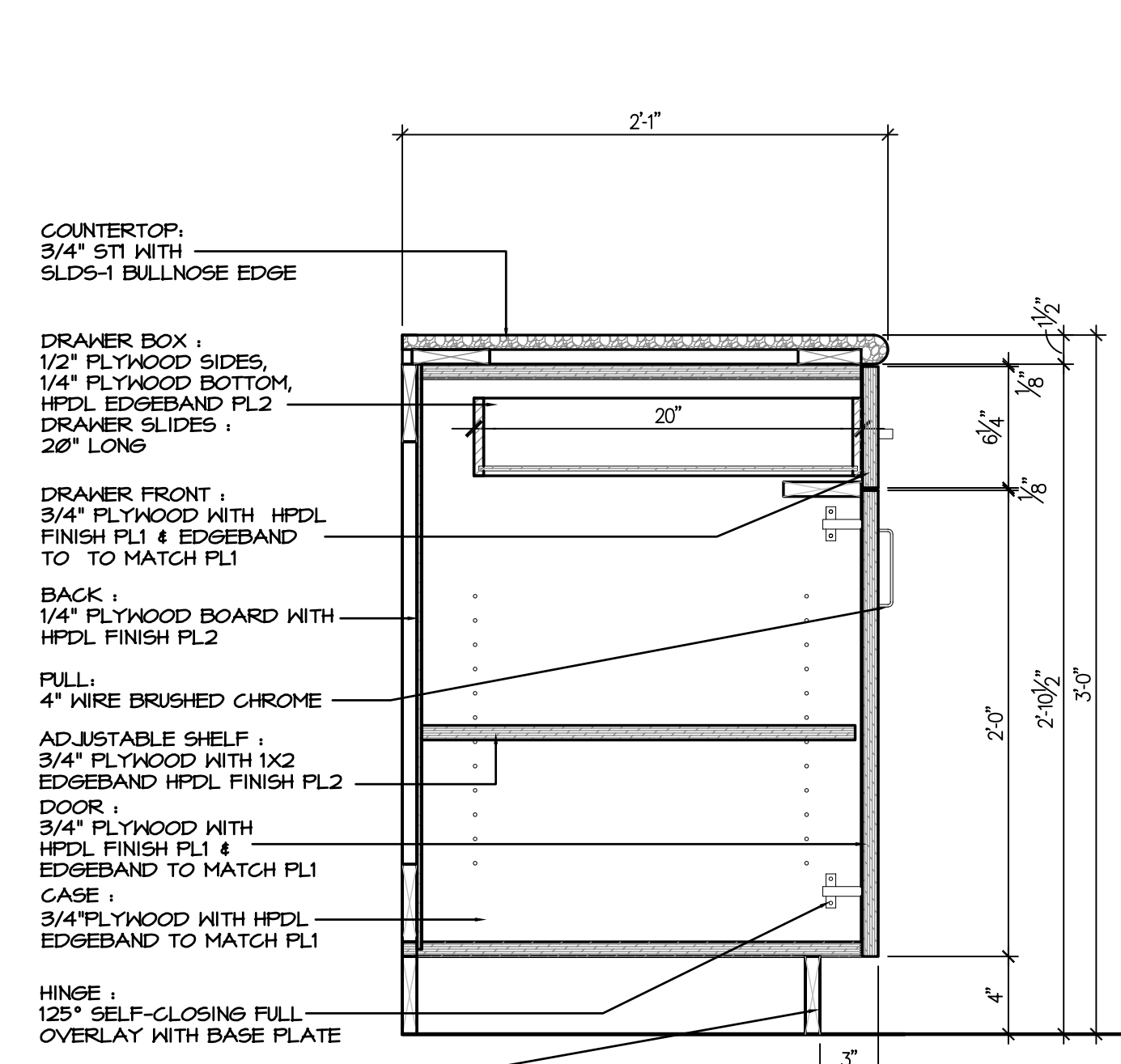
10 MILLWORK SECTION A7.4 SCALE: 1 1/2" = 1'-0"
