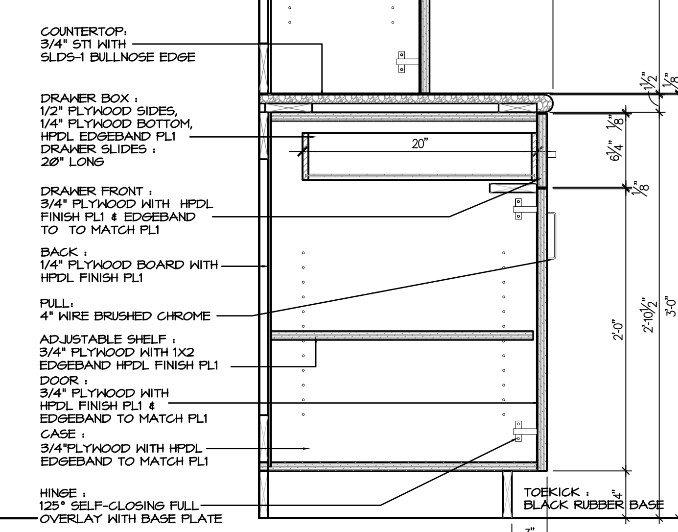
4 MILLWORK SECTION A7.4 SCALE: 1 1/2" = 1'-0"
