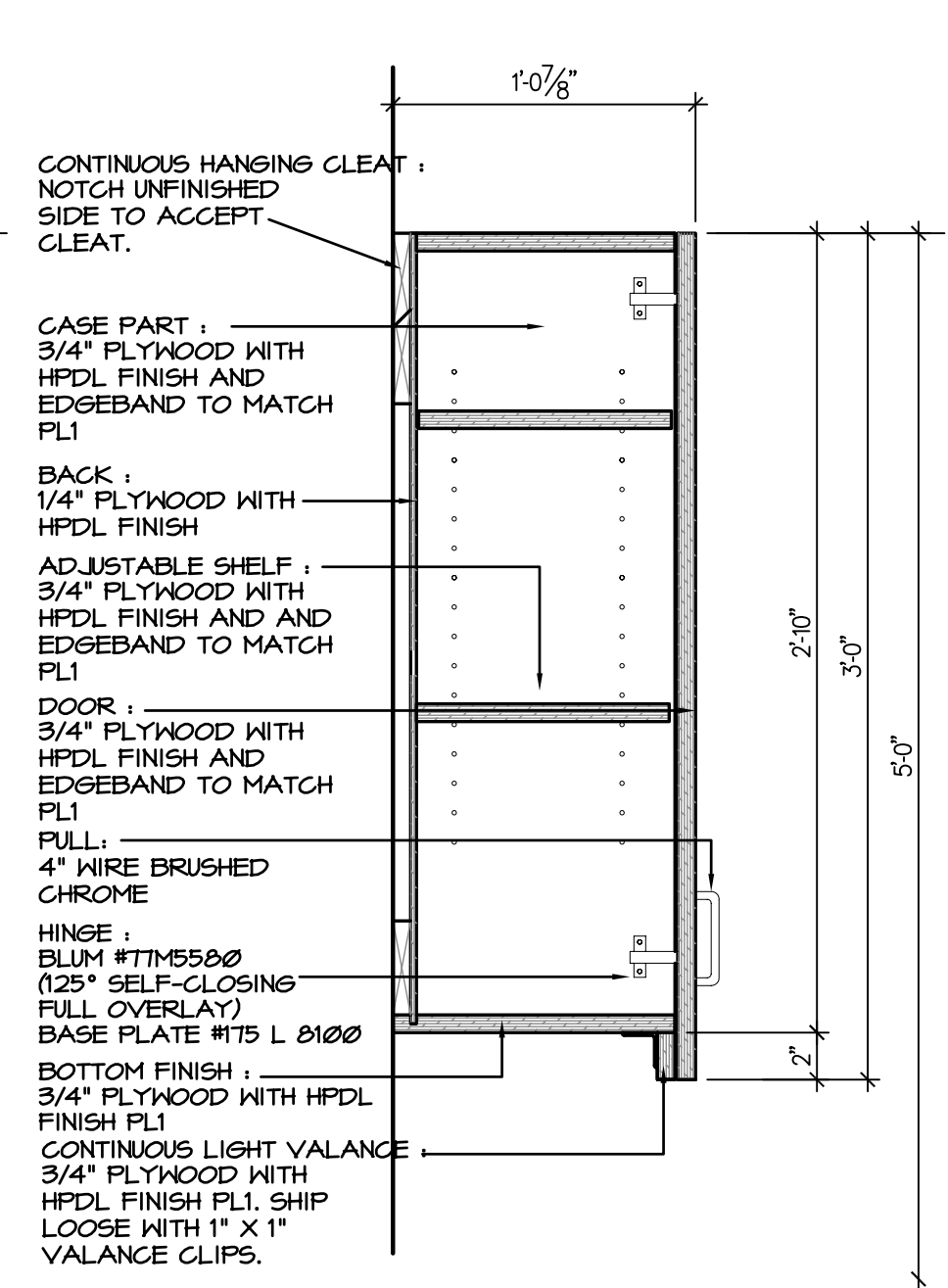
7 MILLWORK SECTION A7.4 SCALE: 1 1/2" = 1'-0"
