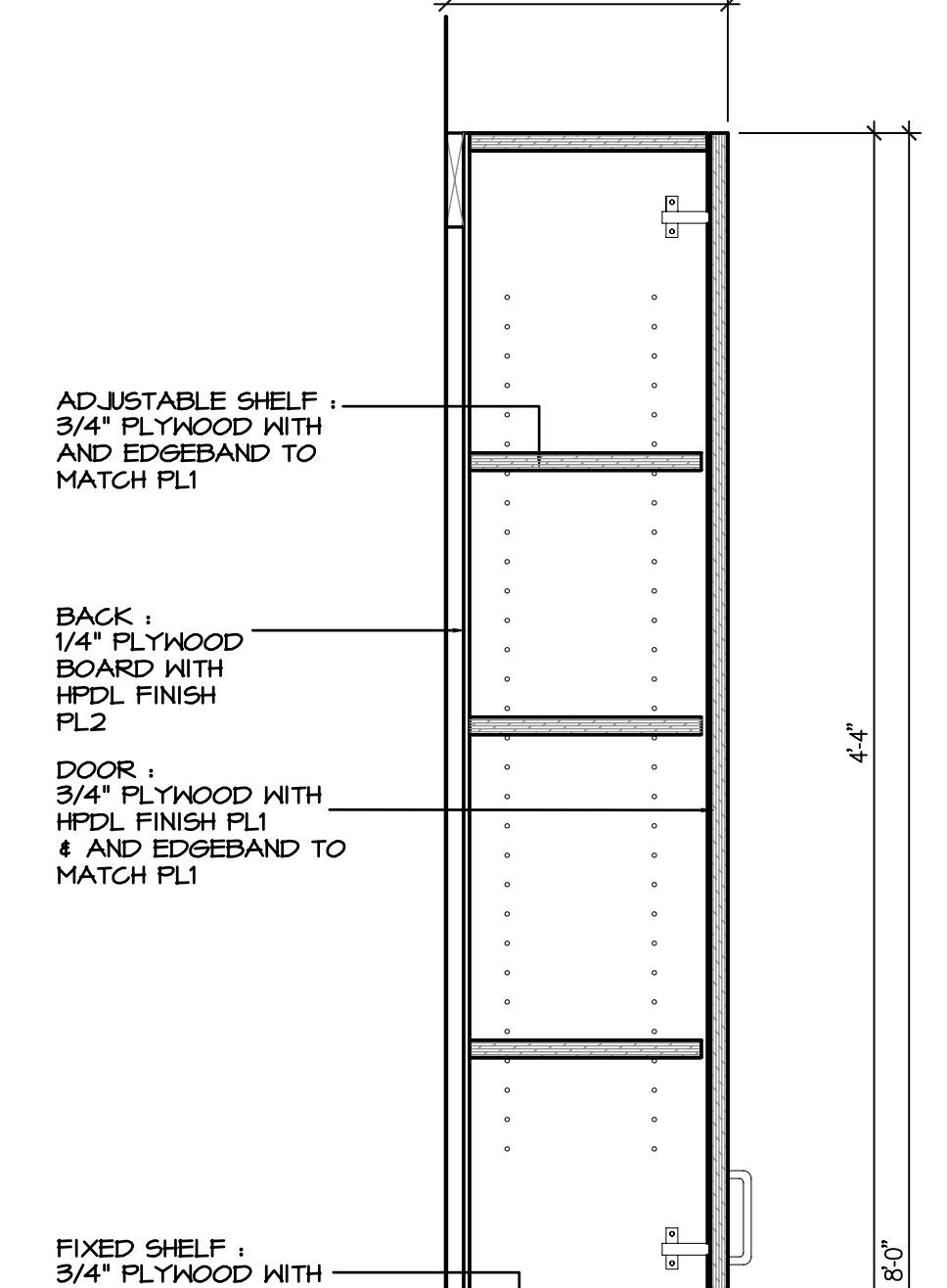
9 MILLWORK SECTION A7.4 SCALE: 1 1/2" = 1'-0"
