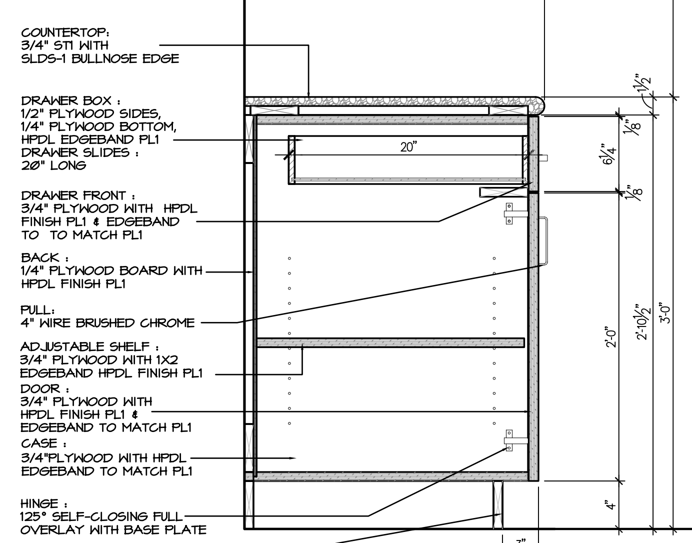
1 MILLWORK SECTION A7.4 SCALE: 1 1/2" = 1'-0"
