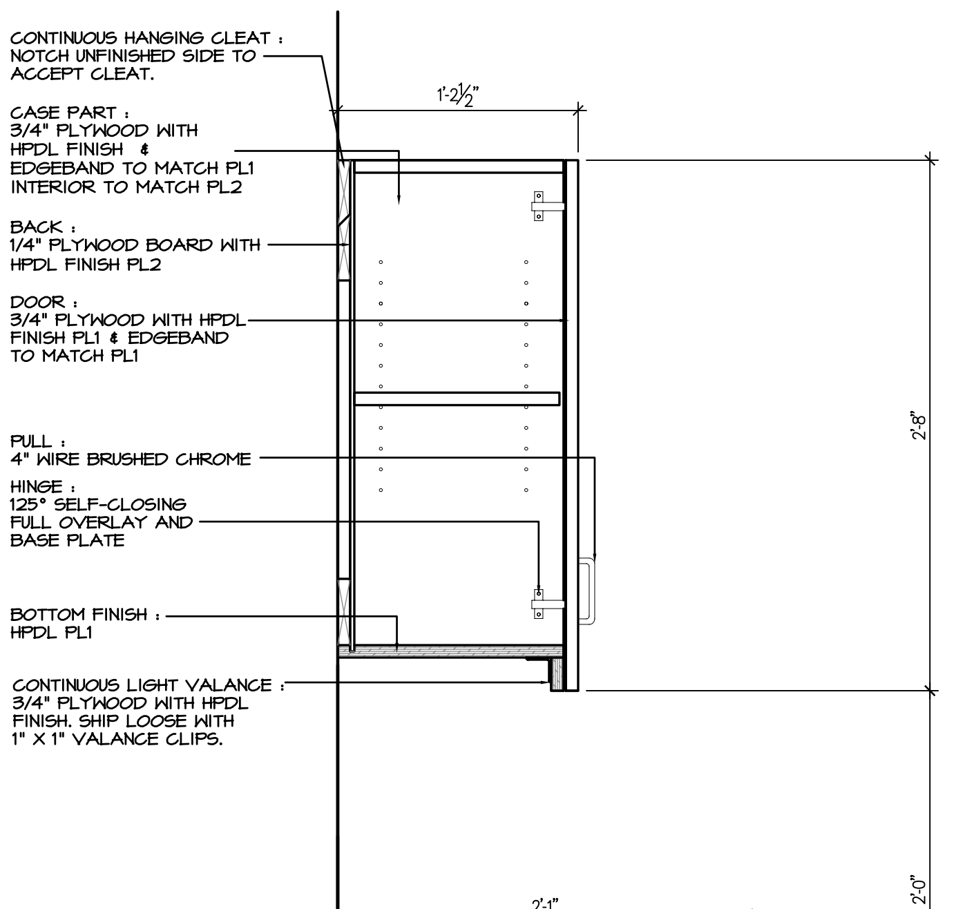
1 MILLWORK SECTION A7.4 SCALE: 1 1/2" = 1'-0"
