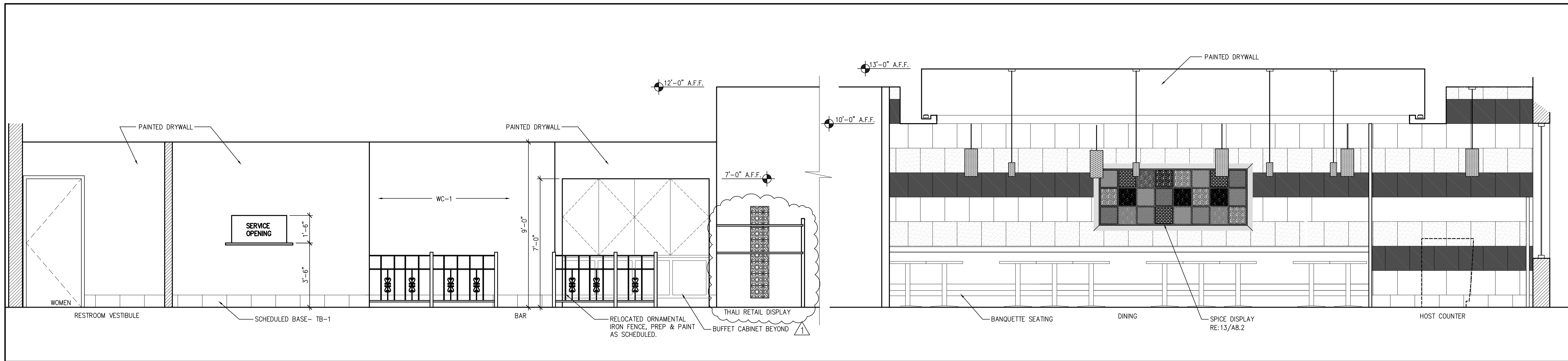
ELEVATION @ HALL & DINING 3/8" = 1'-0" 3
