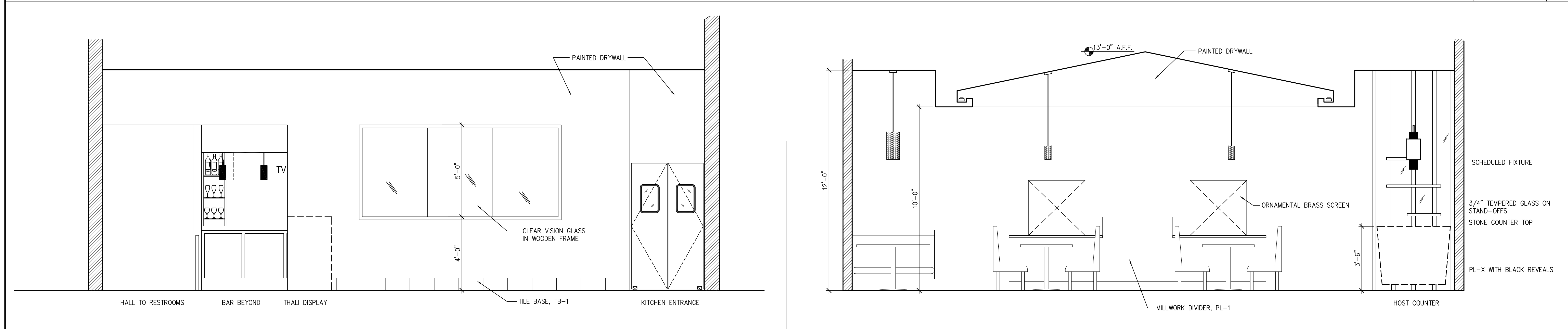
ELEVATION @ DINING & HOST COUNTER 3/8" = 1'-0" 2
