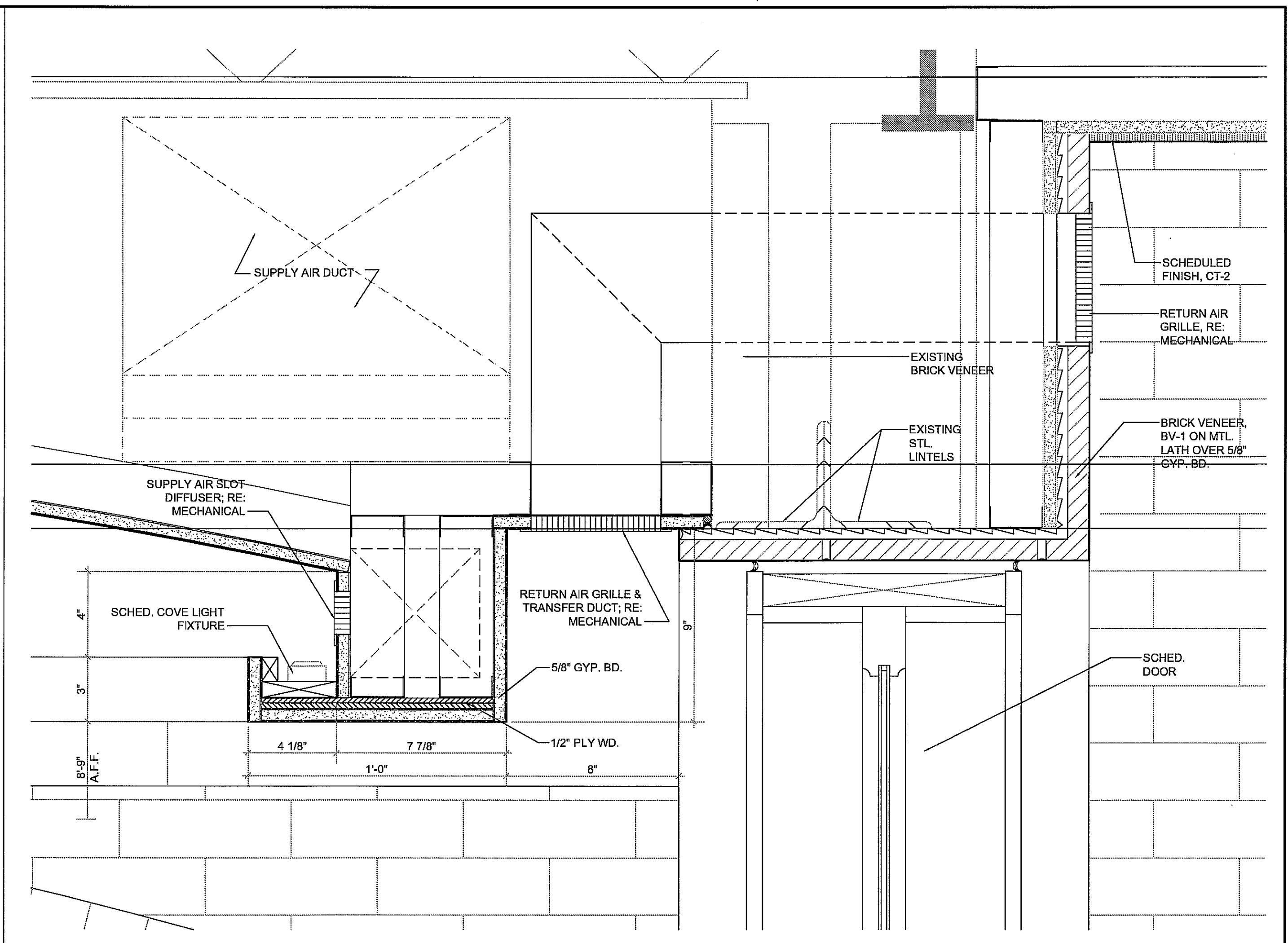
CEILING PRIVATE DINING ENTRY
