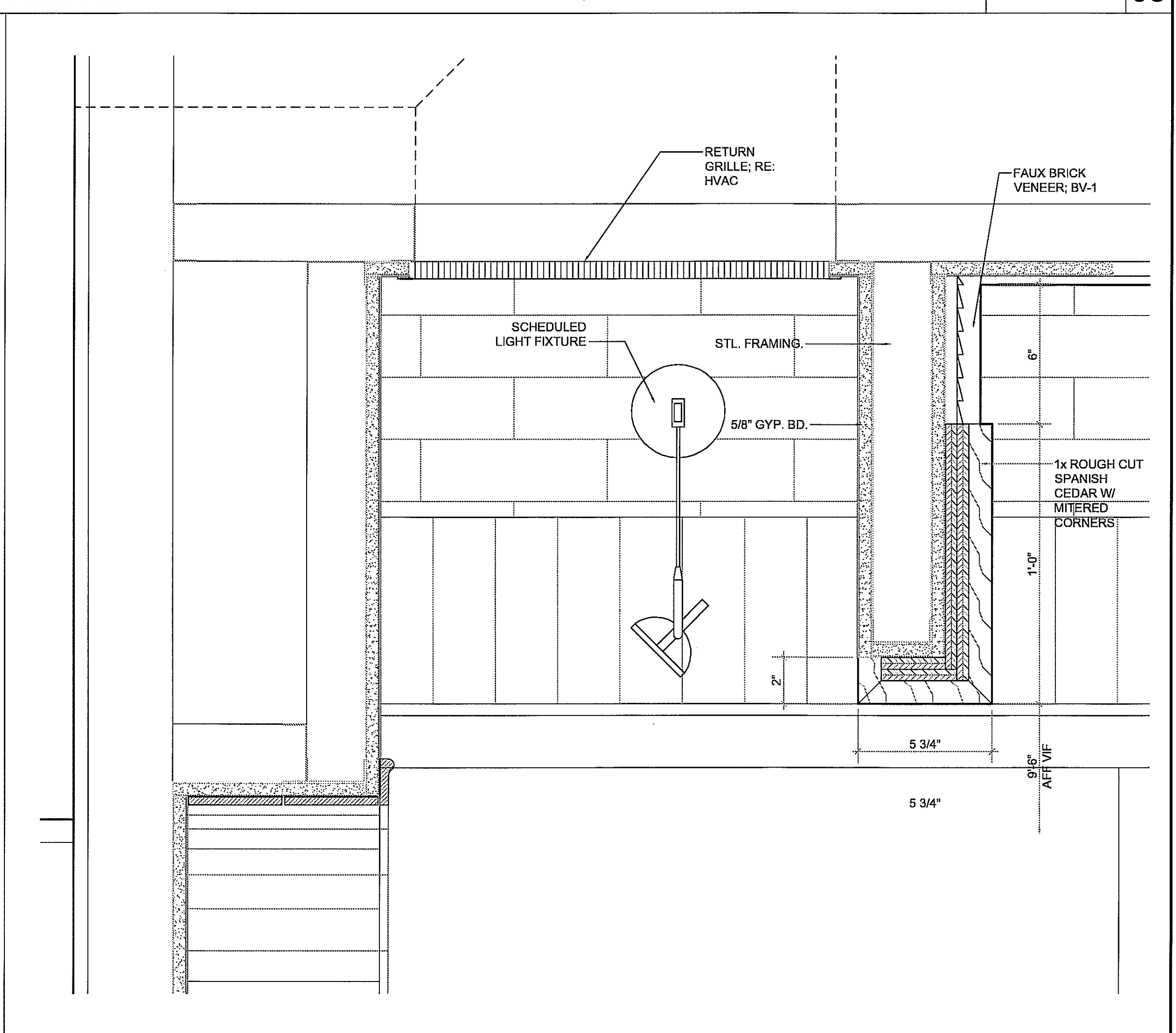
CEILING AT ANTIPASTI
