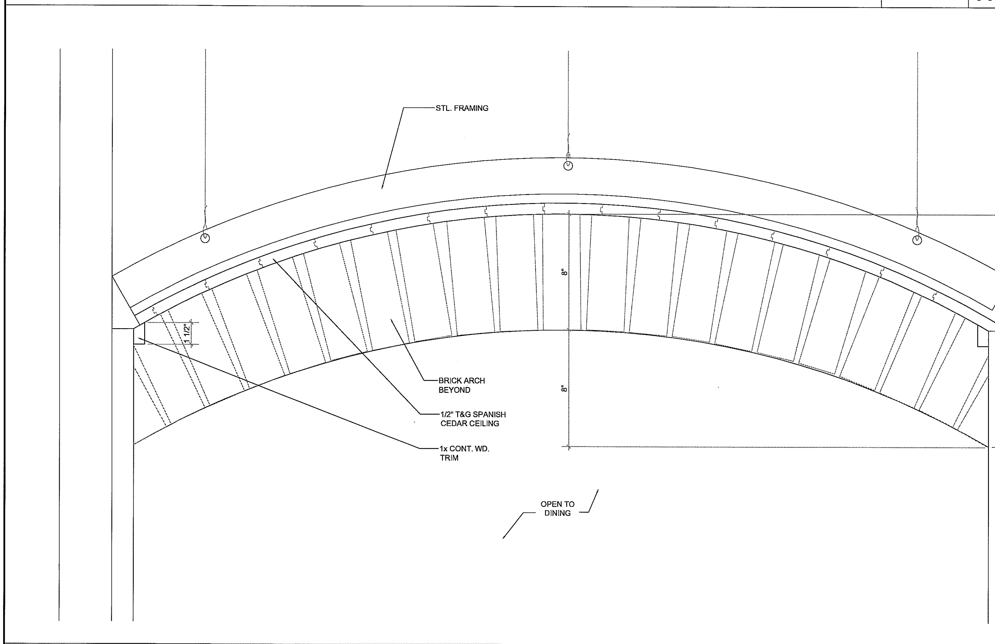
CEILING AT HALL
