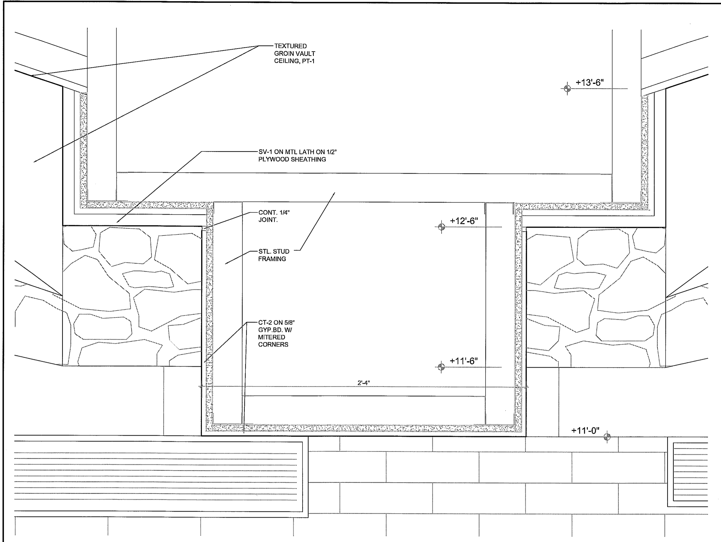
CEILING AT DINING 3" = 1'-0" 15
