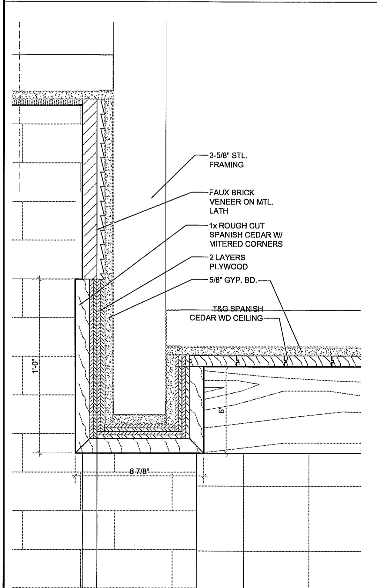
CEILING AT ENTRY/DINING 3" = 1'-0" 17
