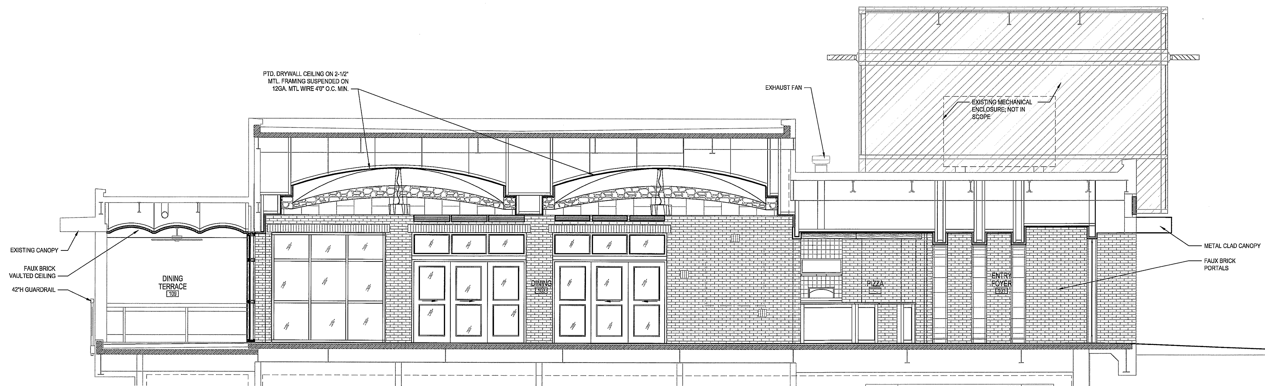
BUILDING SECTION LOOKING SOUTH
