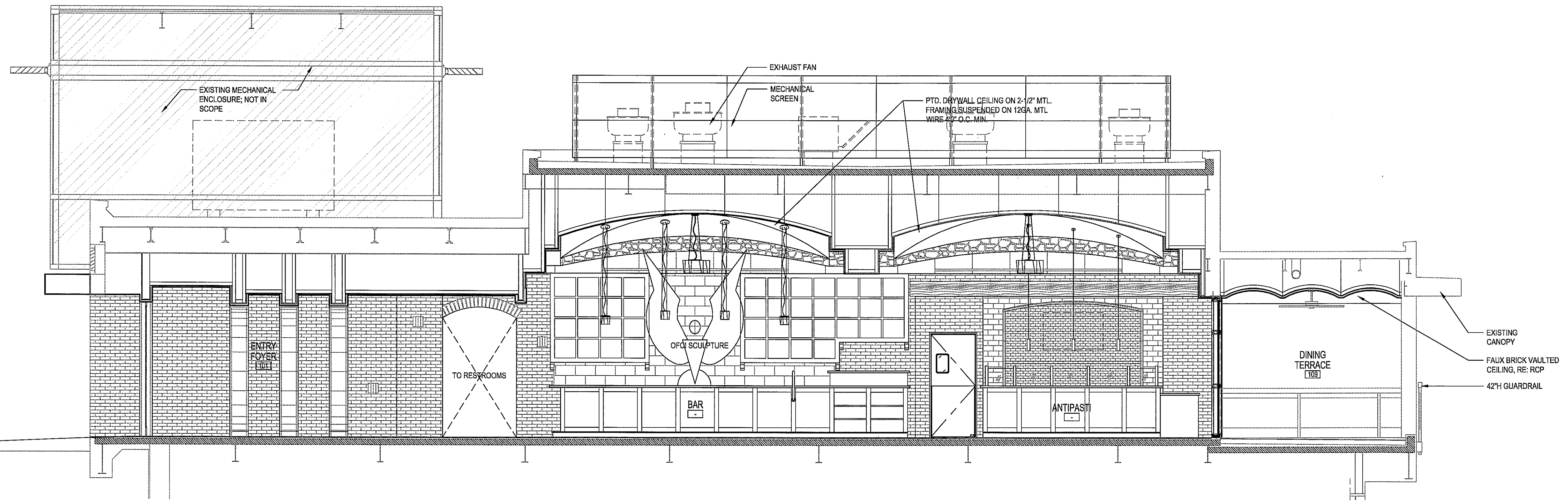
BUILDING SECTION LOOKING NORTH
