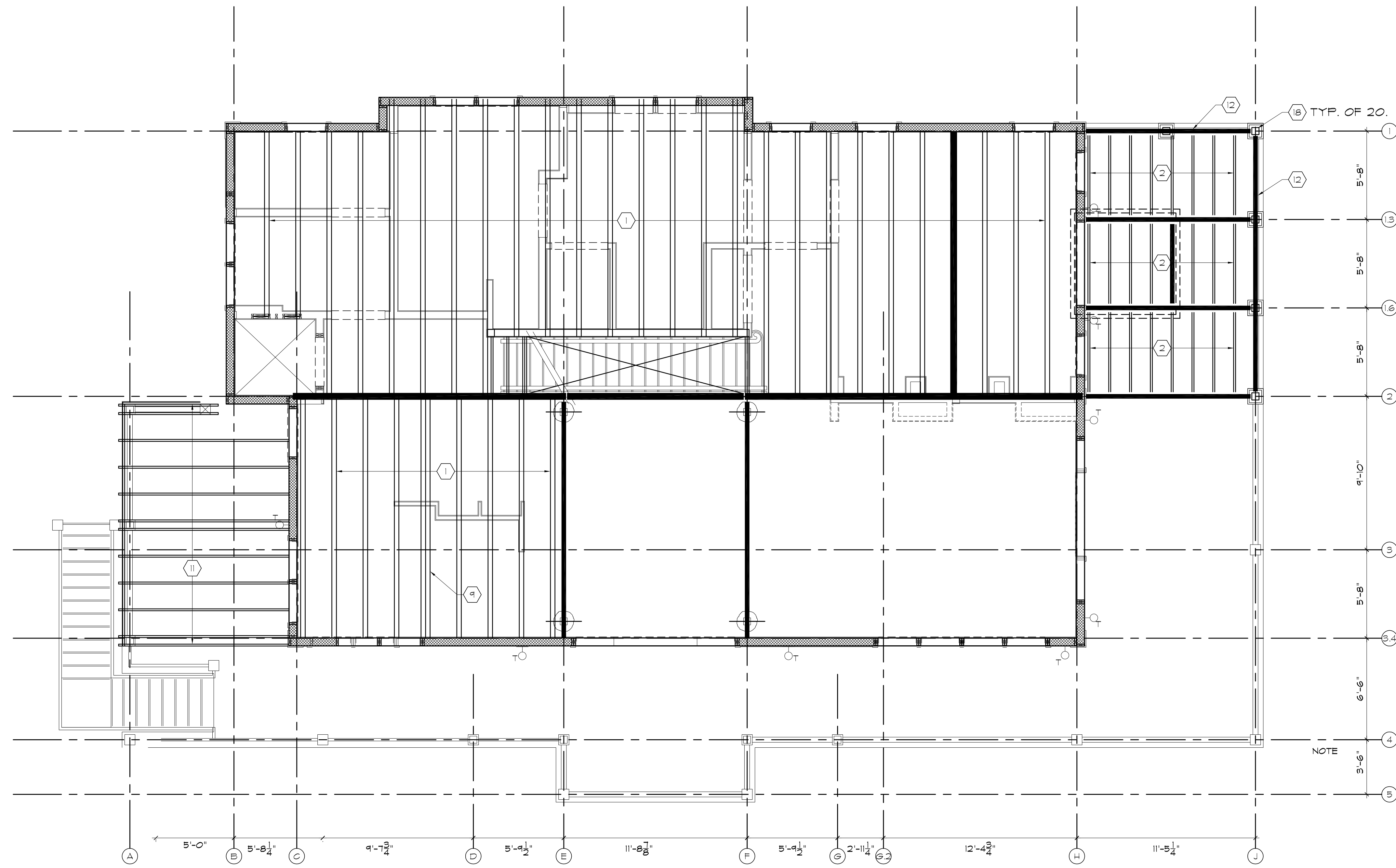
TOWER LEVEL FRAMING PLAN SCALE: 1/4" = 1'-0"
