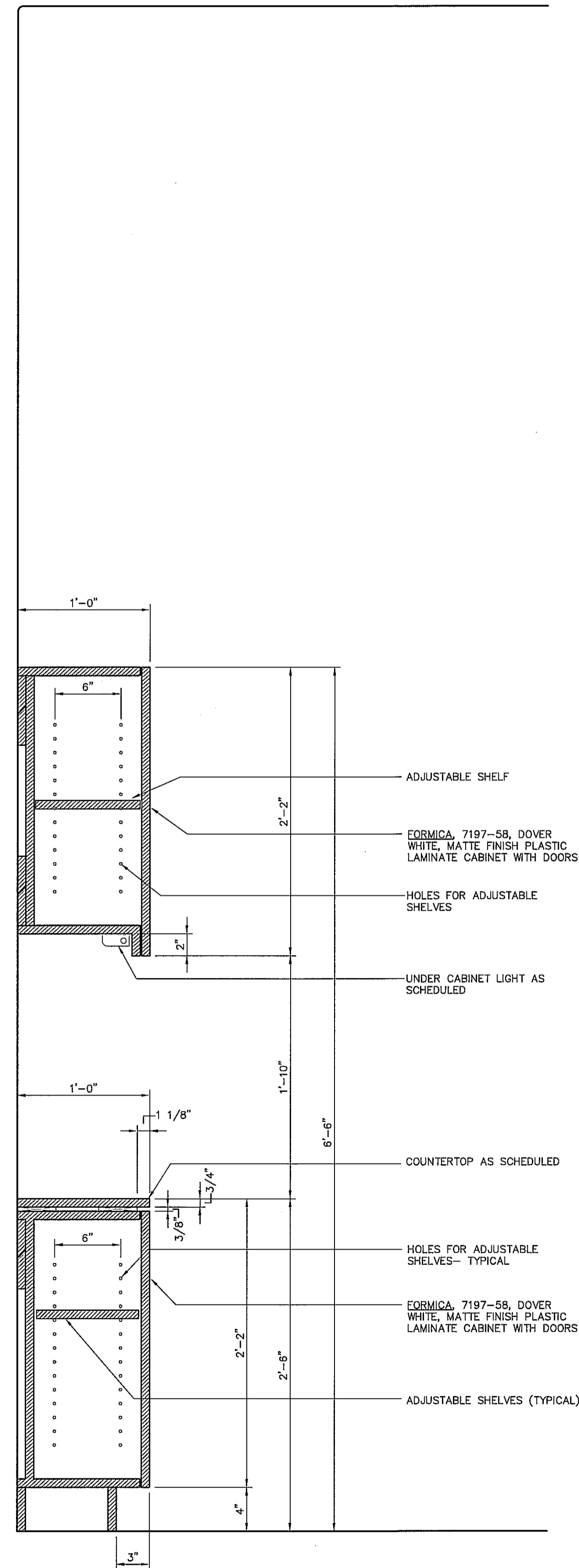
CASEWORK SECTION 02 SCALE:1-1/2"=1'-0"
