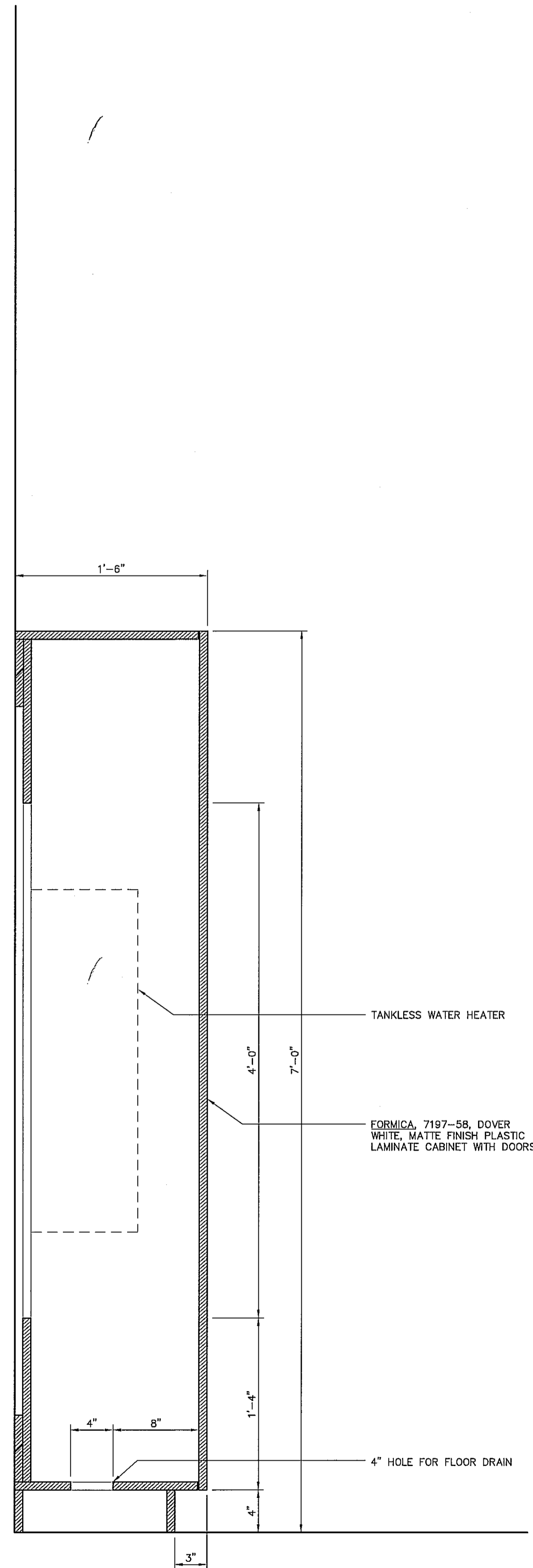
CASEWORK SECTION 03 SCALE:1-1/2"=1'-0"
