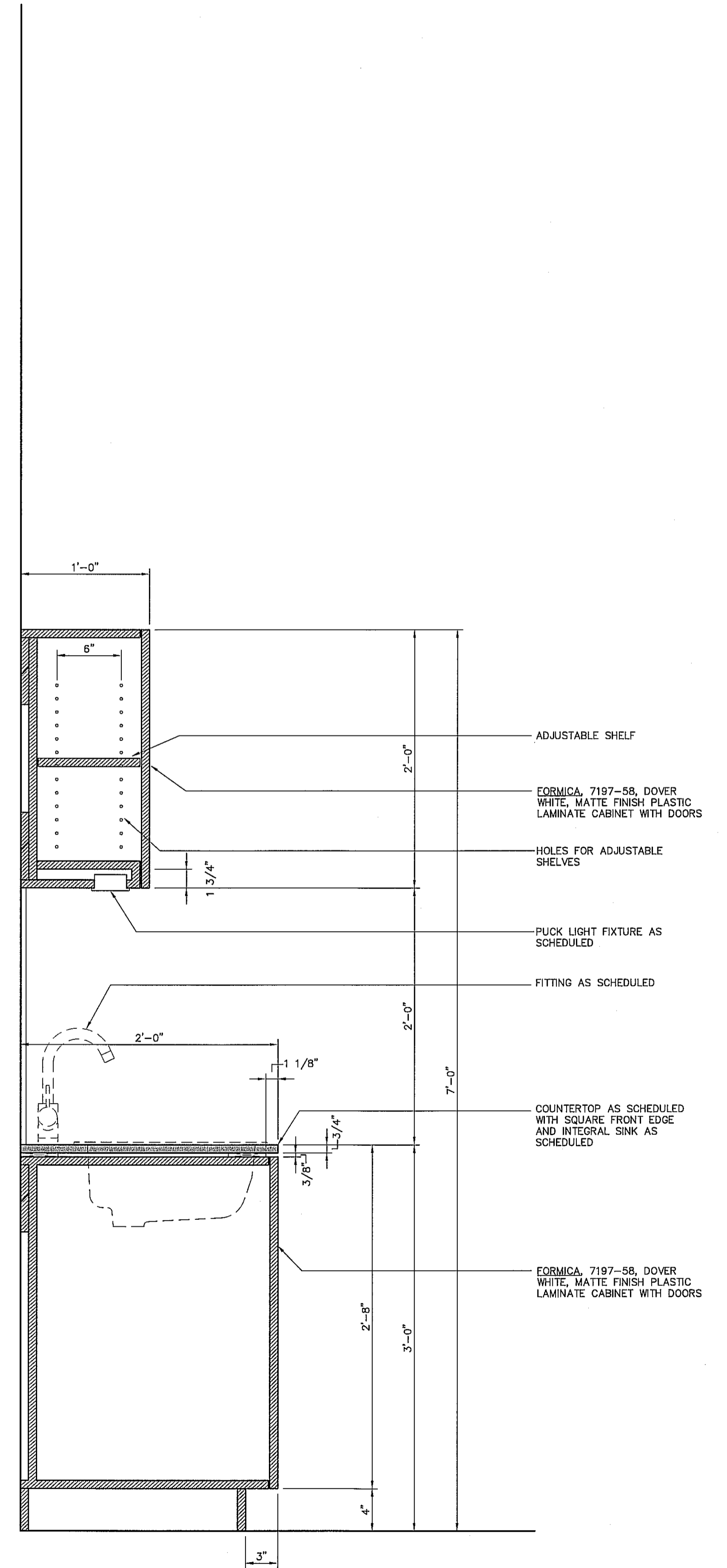
CASEWORK SECTION 01 SCALE:1-1/2"=1'-0"
