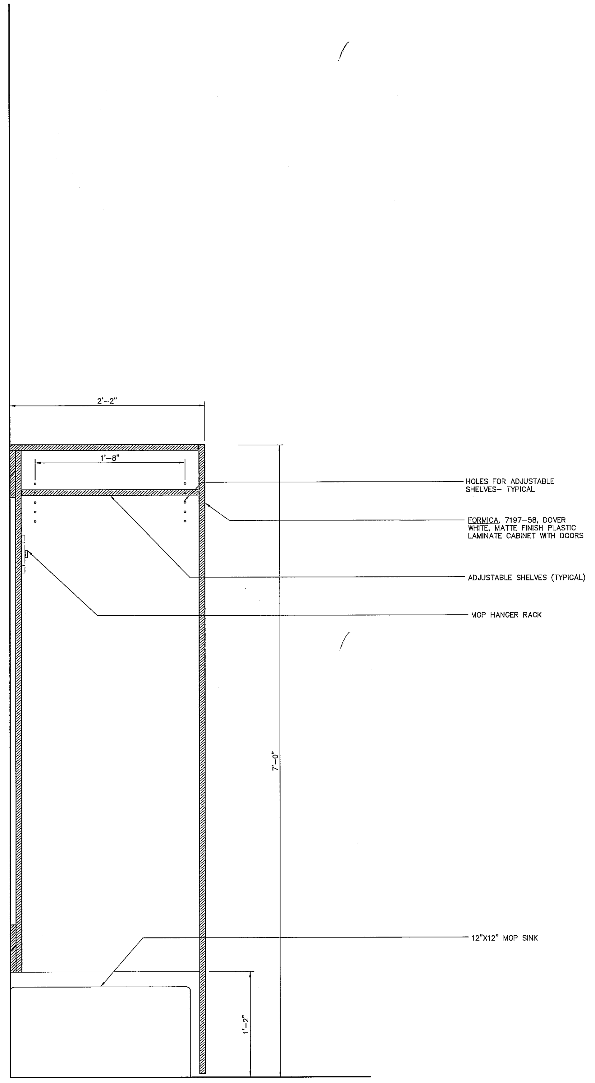
MILLWORK SECTION 03 SCALE: 1-1/2"=1'-0"
