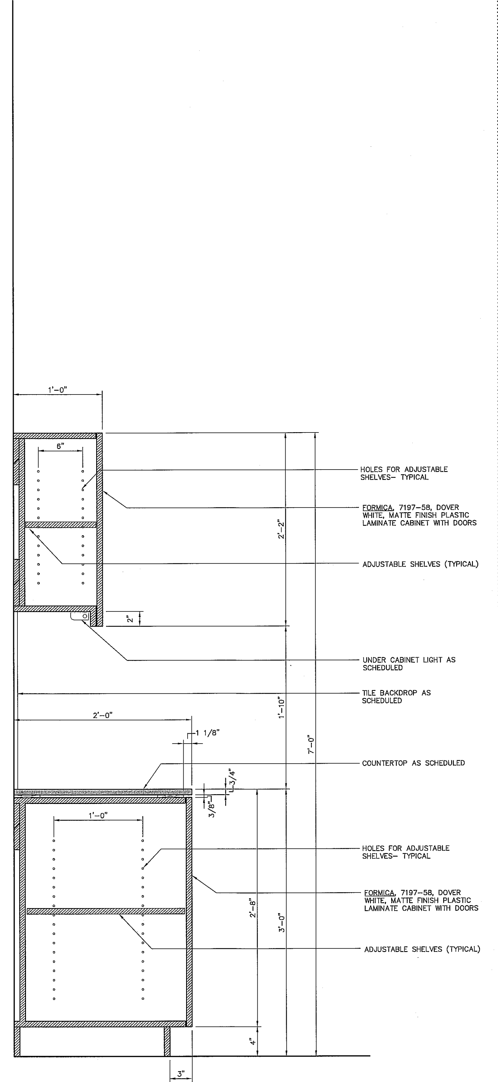
MILLWORK SECTION 01 SCALE: 1-1/2"=1'-0"
