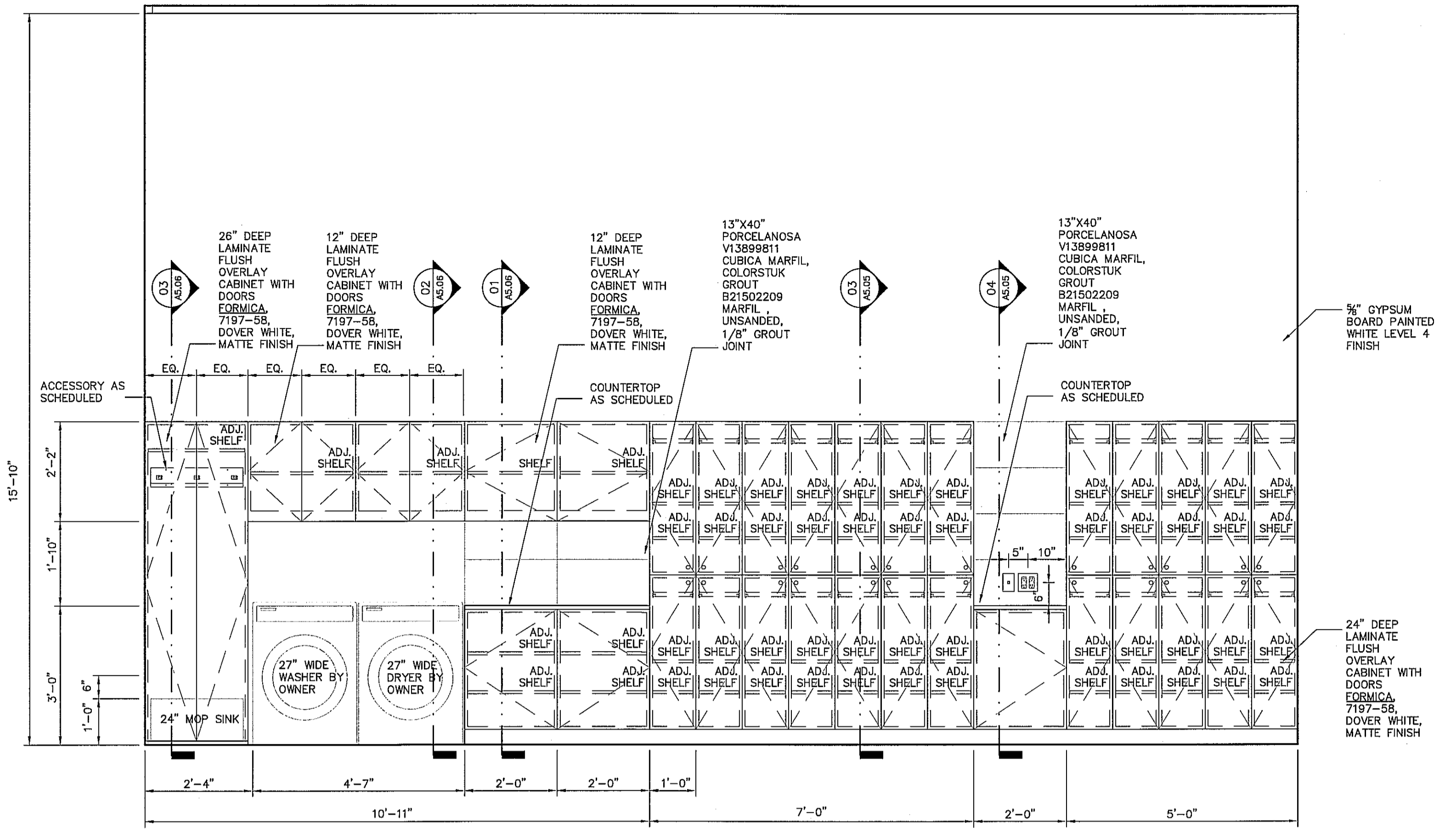
LOCKER/LAUNDRY ROOM ELEVATION 02 SCALE: 1/2"=1'-0"
