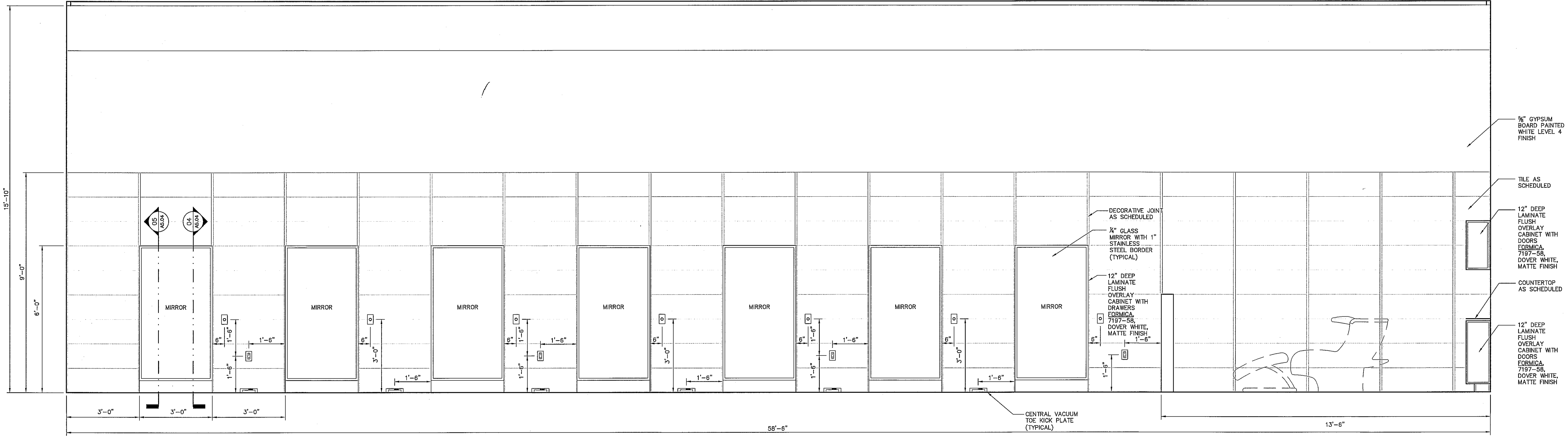
STYLING SHAMPOO ELEVATION ELEVATION 01 SCALE: 1/2"=1'-0"
