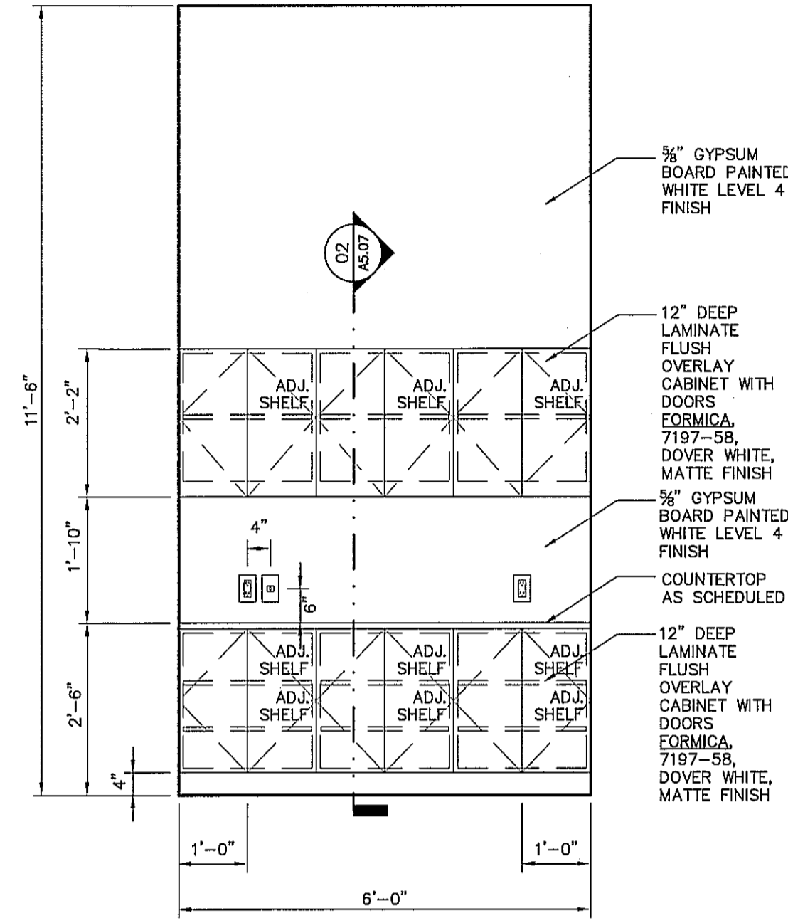
OFFICE ELEVATION 03 SCALE: 1/2"=1'-0"
