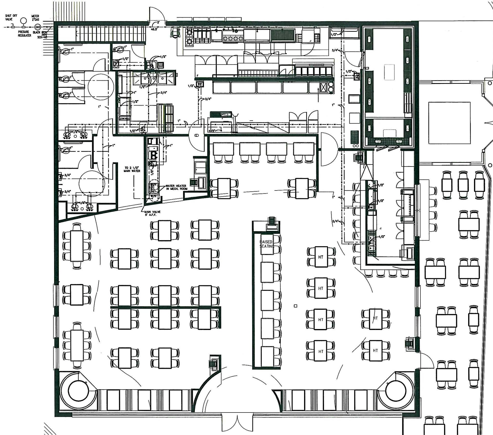
PLUMBING PLAN - WATER & GAS
