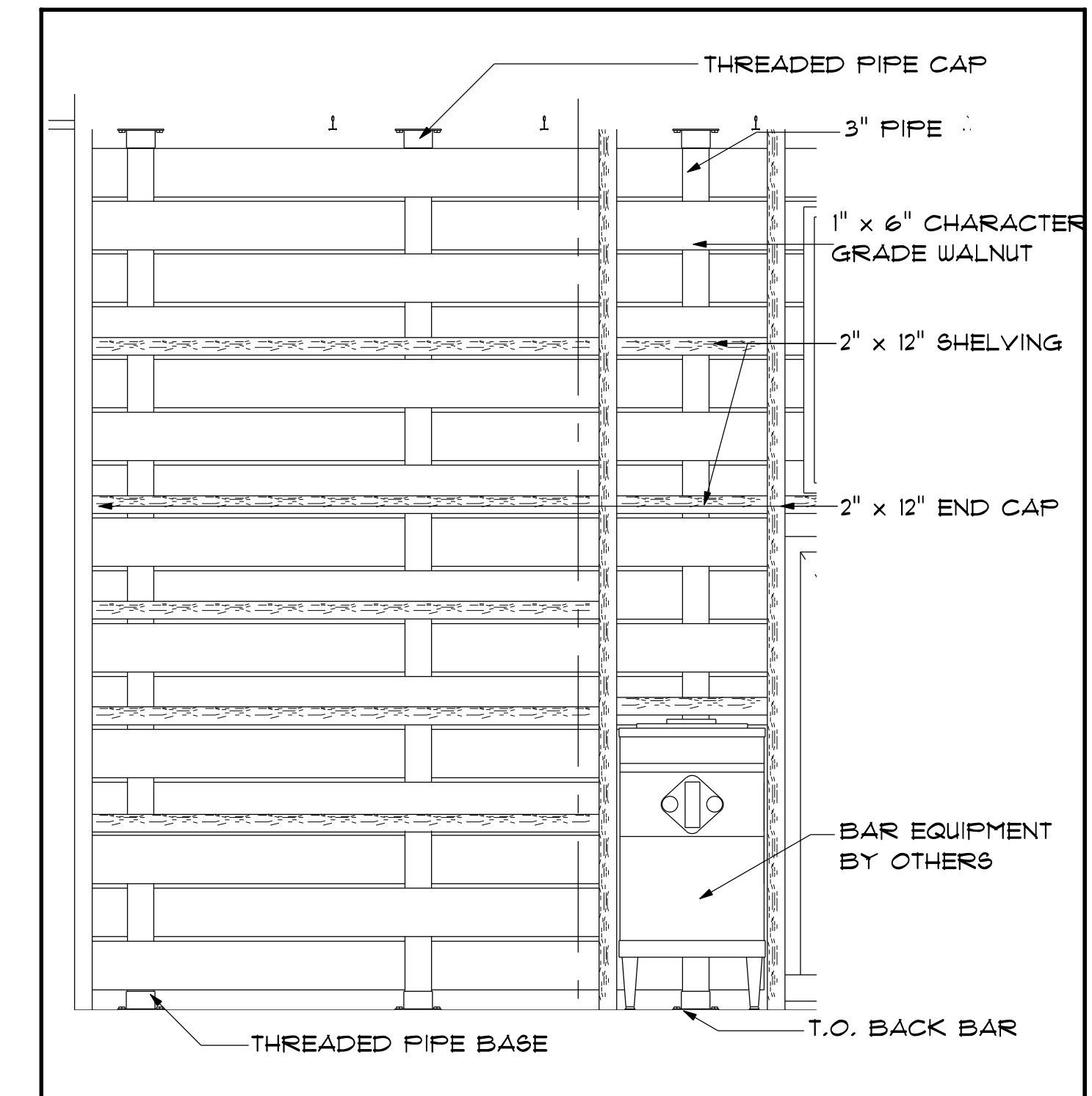
BAR BACK DETAIL
