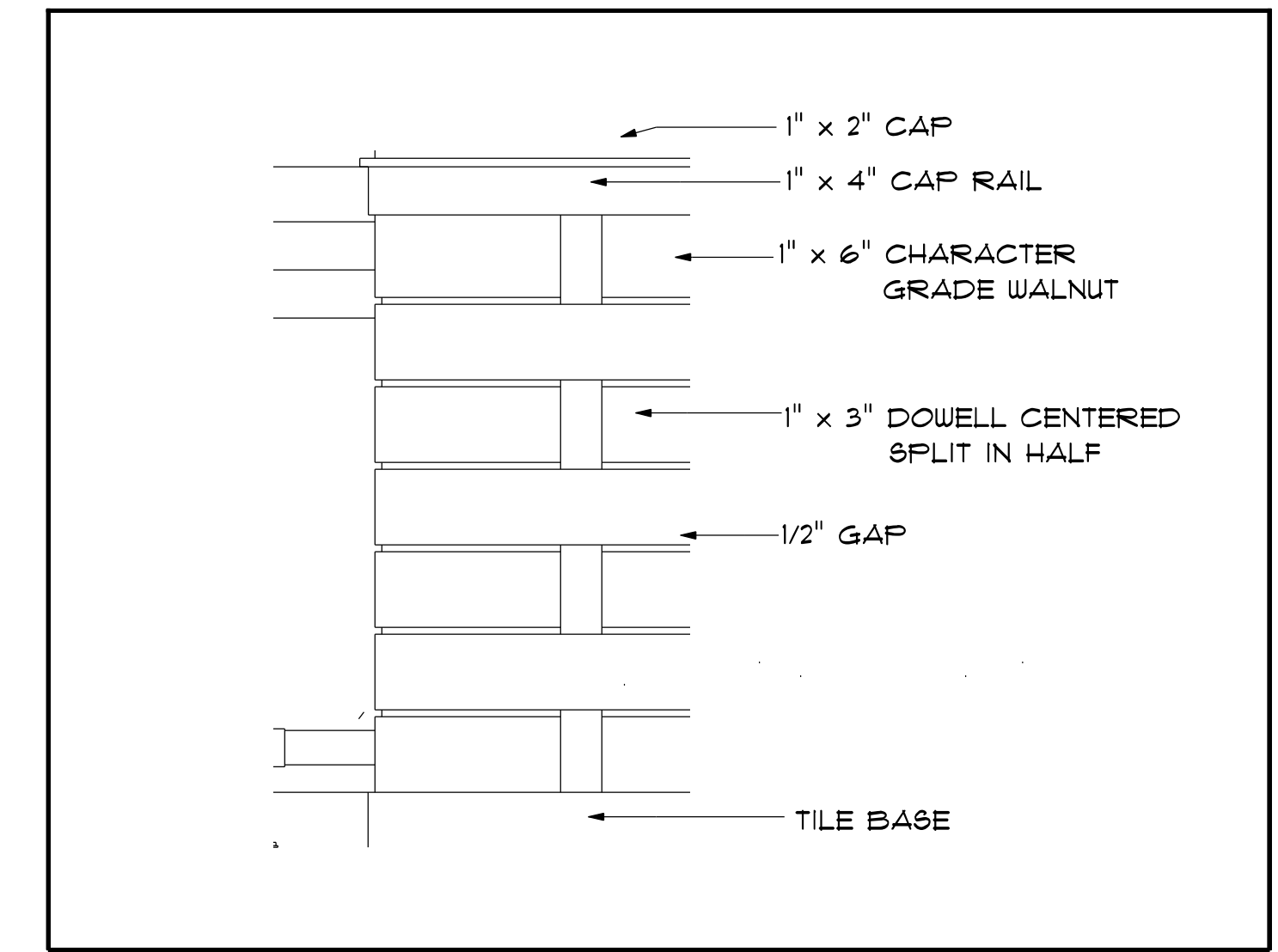
WAINSCOT DETAIL
