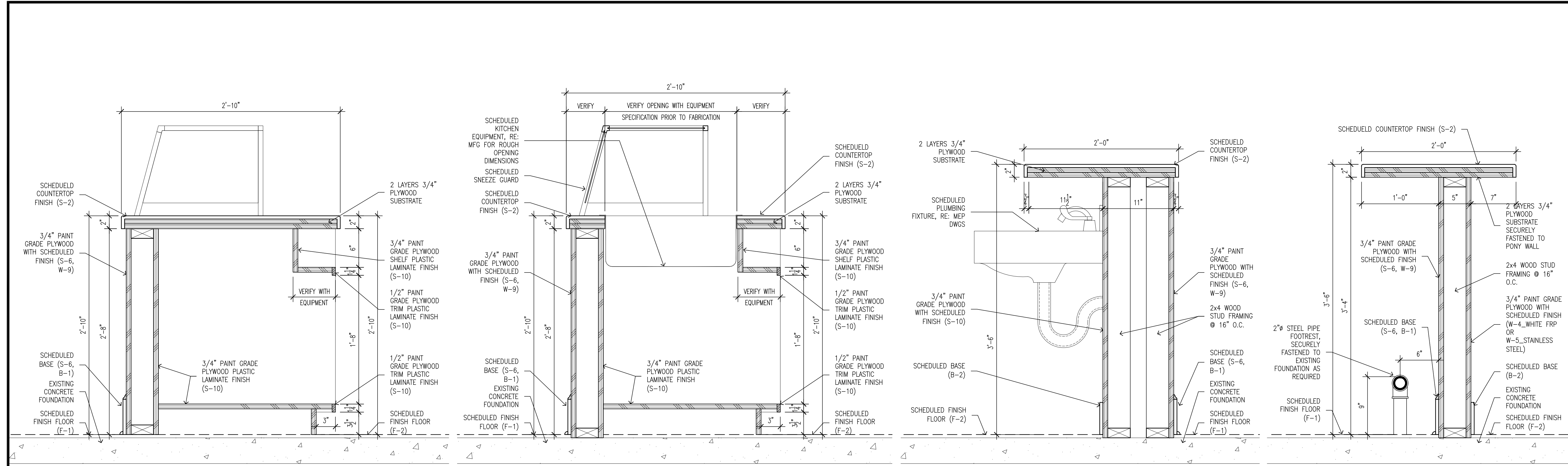
14 A9.0 MILLWORK DETAIL 1-1/2"x1'-0"
