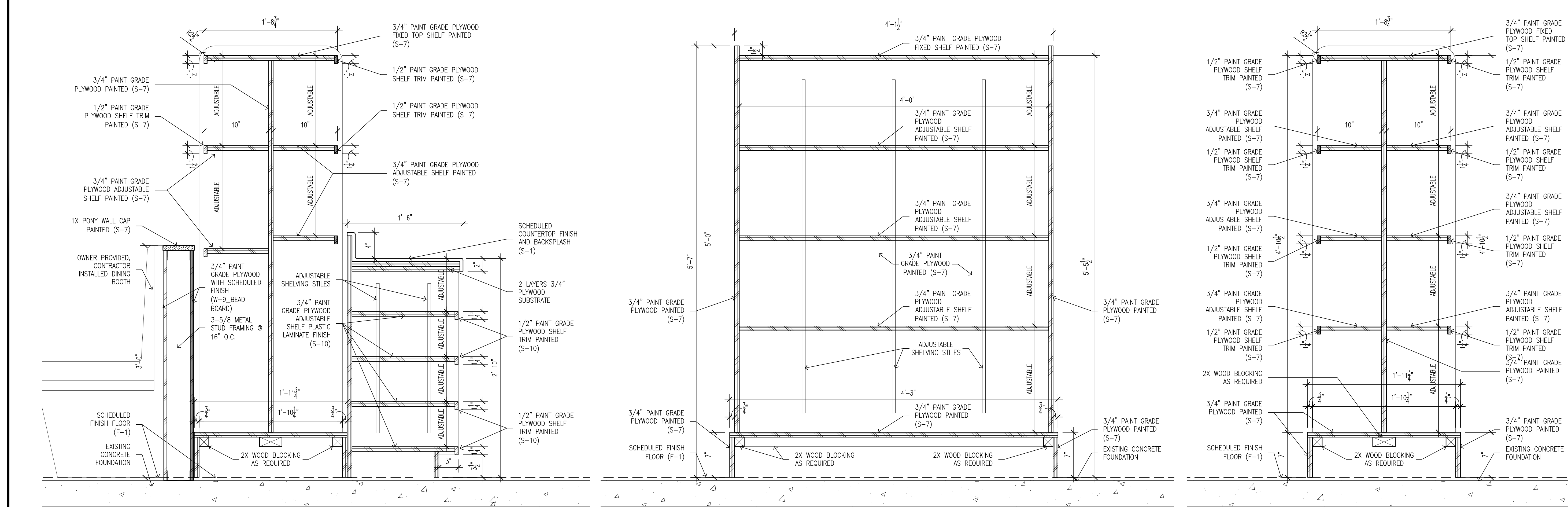
12 A9.0 MILLWORK DETAIL 1-1/2"x1'-0"
