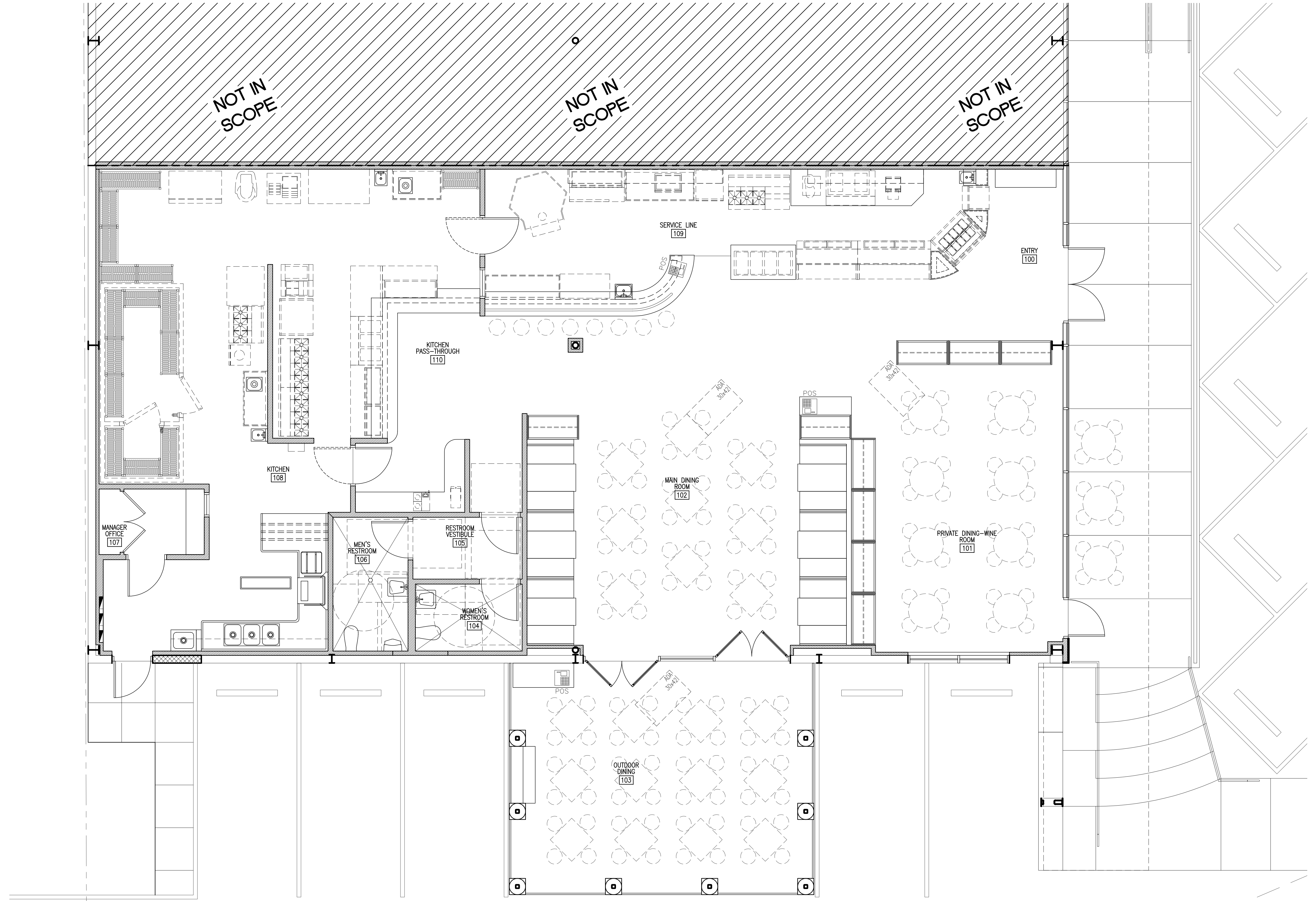
1 A2.2 PROPOSED FURNITURE AND ADA CLEARANCE PLAN 1/4"=1'-0"
