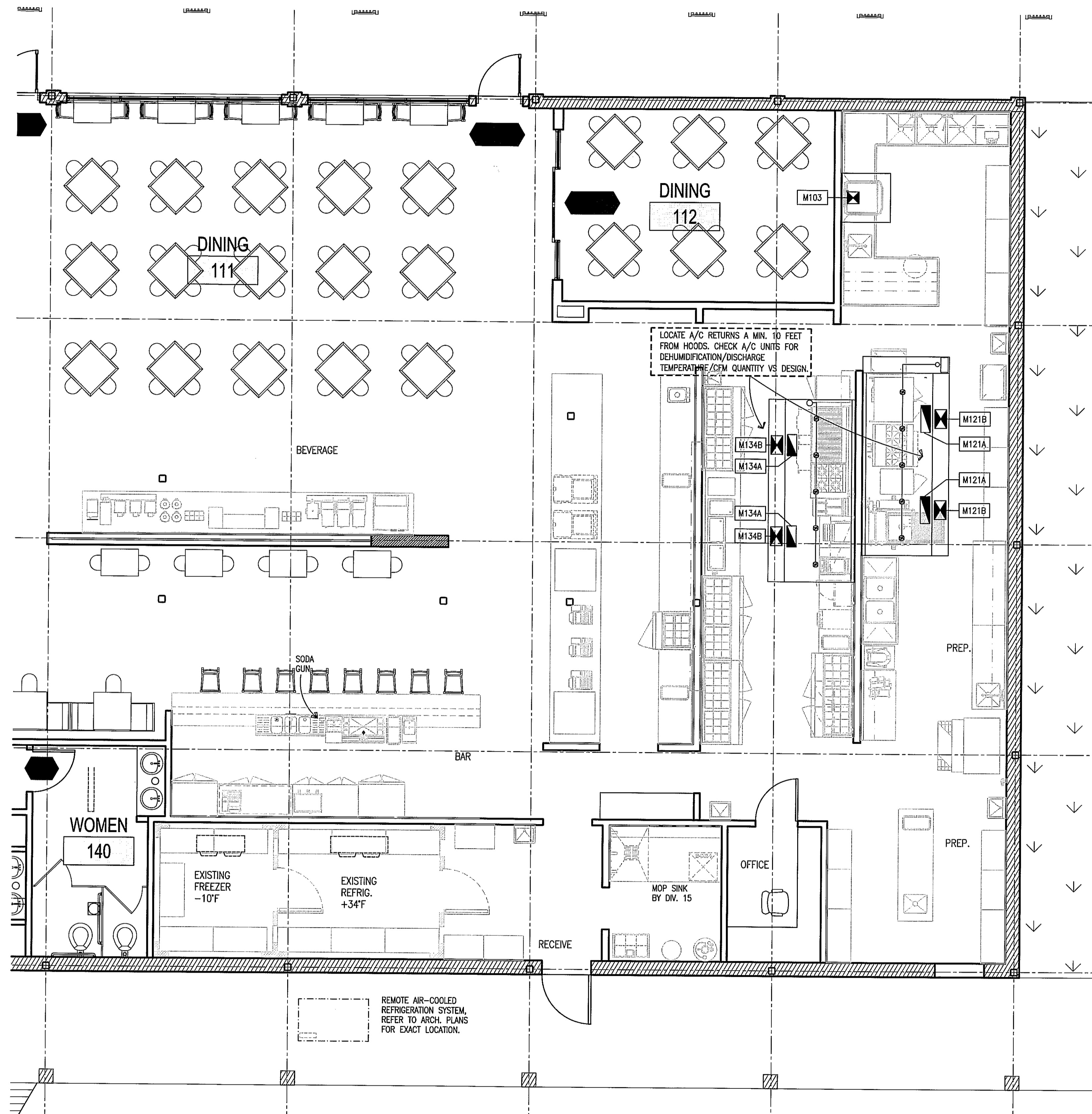
A FS1.4 FOODSERVICE MECHANICAL PLAN SCALE: 1/4"=1'-0"
