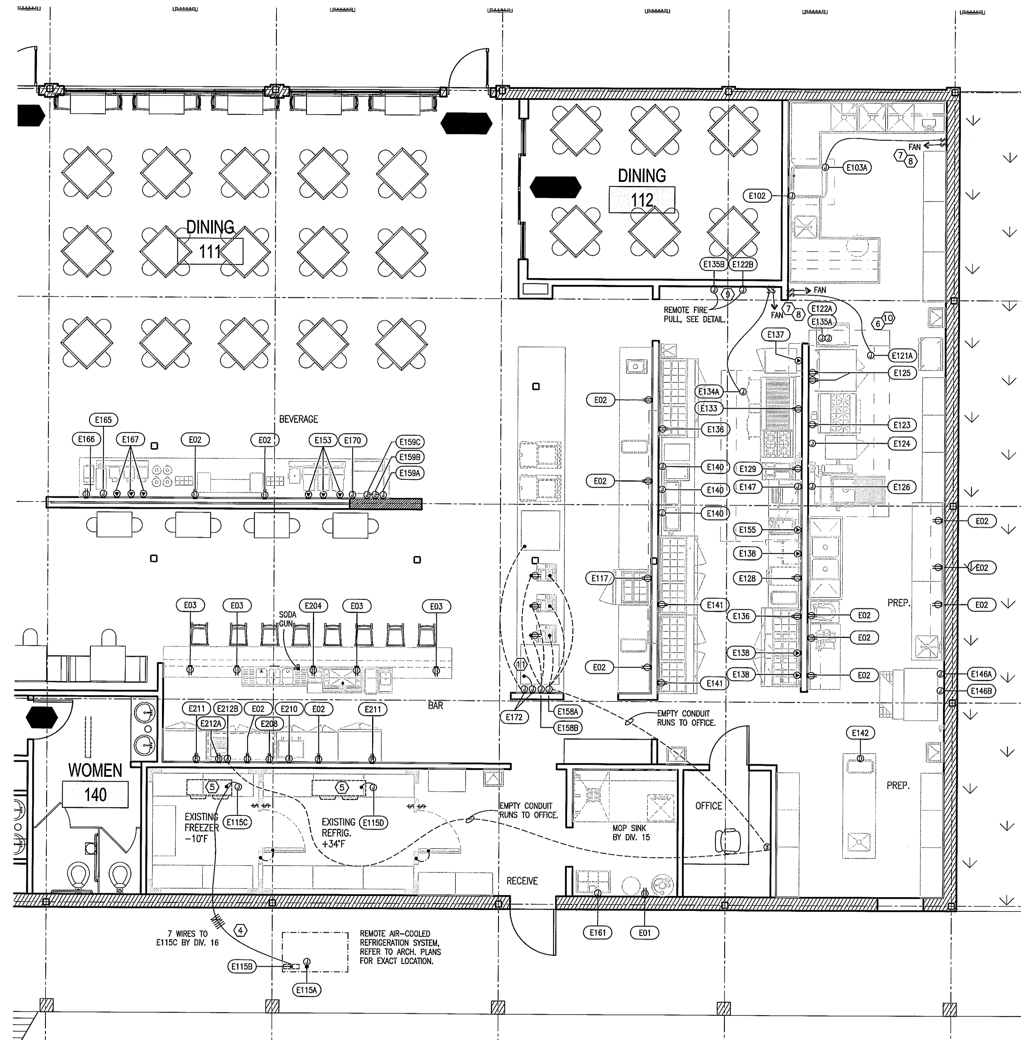
A FOODSERVICE ELECTRICAL PLAN FS1.3 SCALE: 1/4"=1'-0"
