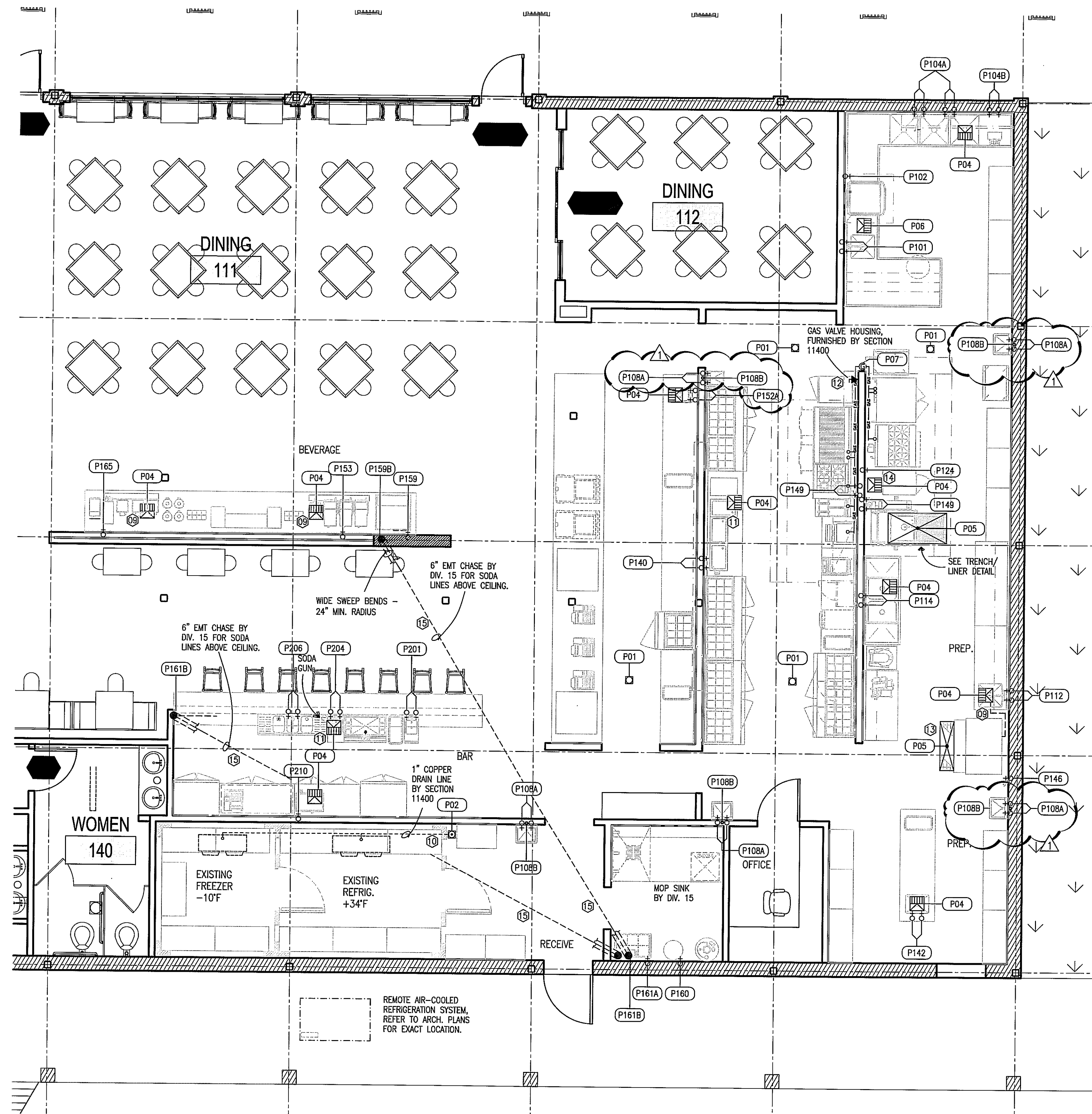
A FOODSERVICE PLUMBING PLAN FS1.2 SCALE: 1/4"=1'-0"
