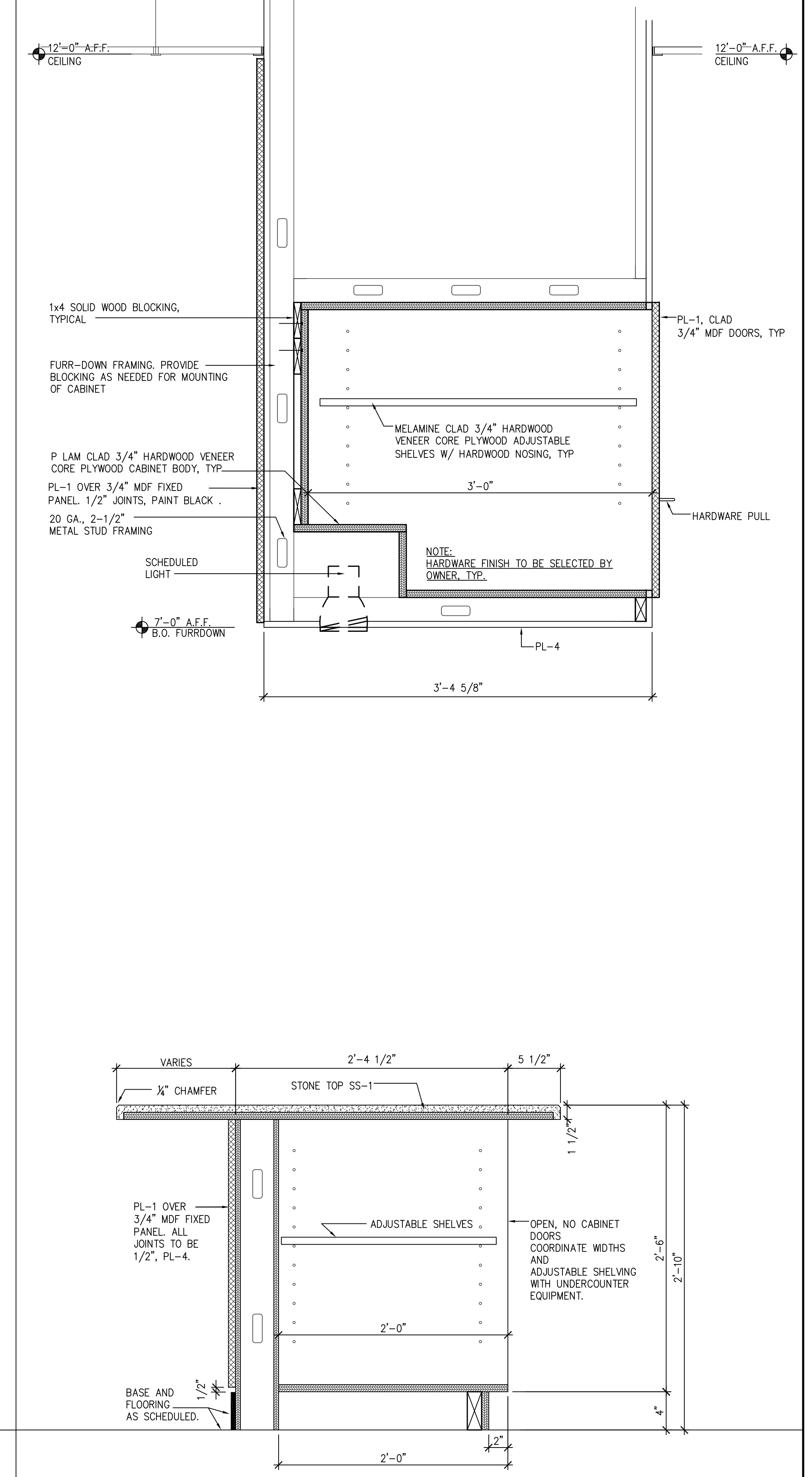
SECTION @ PICK-UP
